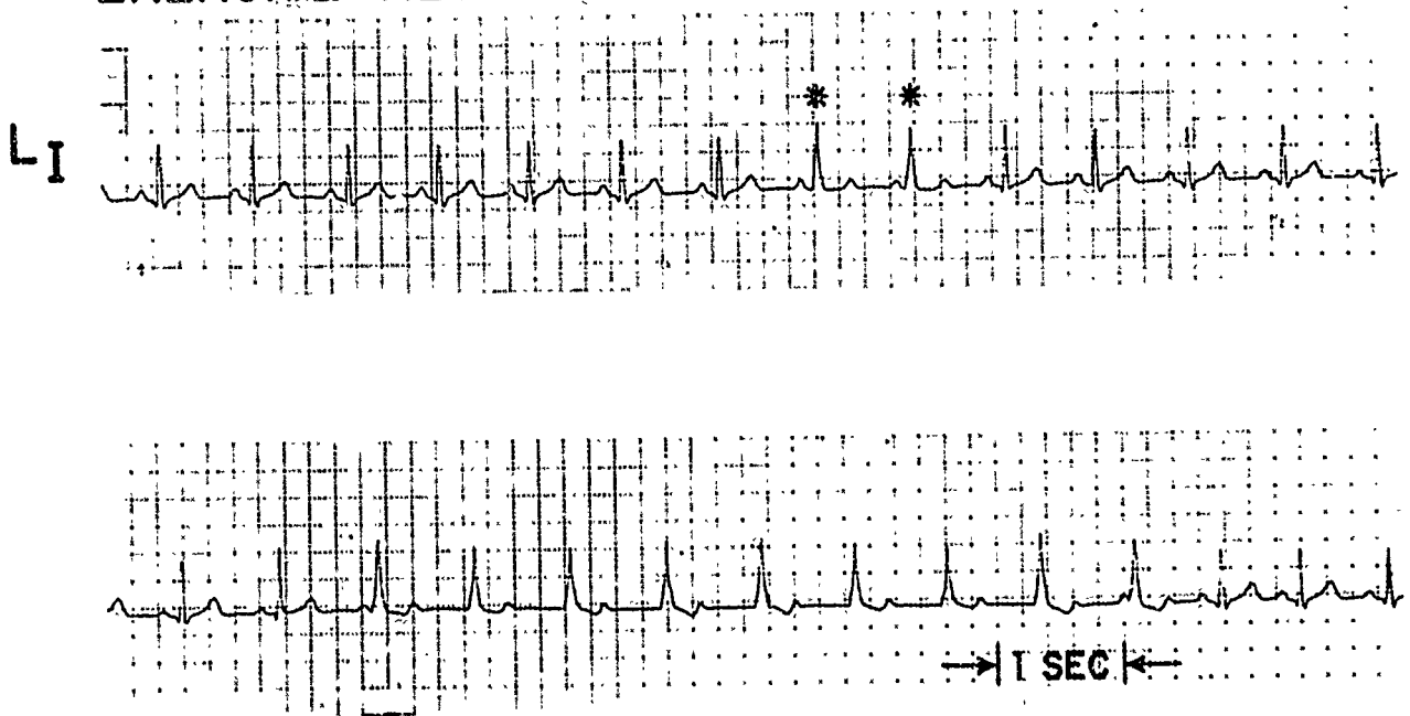
Fig. 6. Wandering pacemaker with fusion beats (designated with asterisk) and dominant low nodal rhythm. See text for discussion
