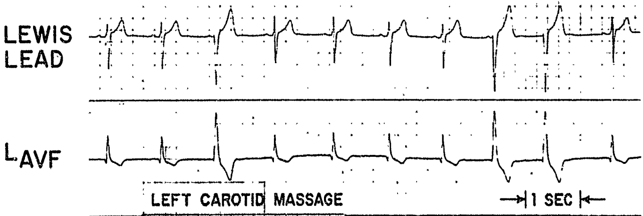
Fig. 7. Sinus bradycardia with wandering pacemaker accentuated with edrophonium chloride and carotid sinus massage in Patient No. ...
