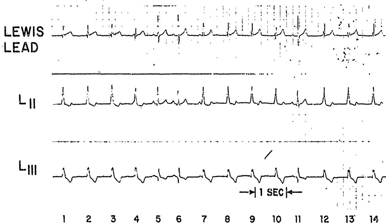
Fig. 5. Wandering pacemaker demonstrated in Patient No. 2 in several simultaneous leads during the recovery from Valsalva maneuver. See text for discussion.
