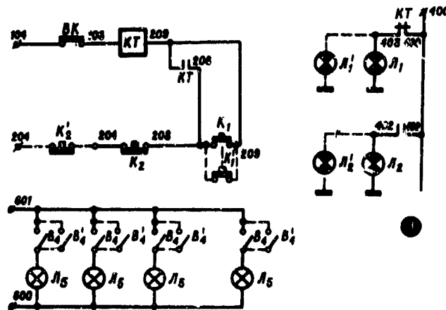
Fig. 3. Diagram of PTP-180 remote control panel. Dotted line shows the changes made in the basic diagram.
