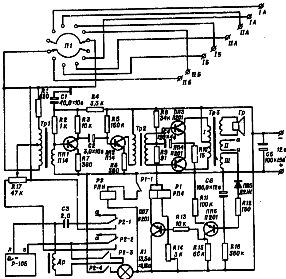
Basic electrical circuit of a device for coupling radio and radio-relay sets. KEY: a -- R-105
