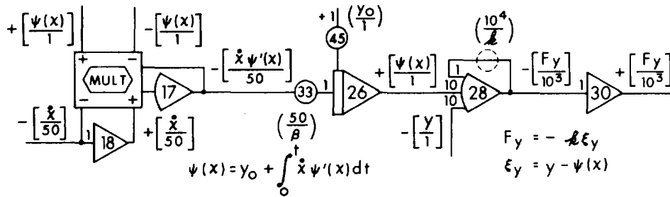
Figure 6. Diagram for Generating \psi(x) and F_y
