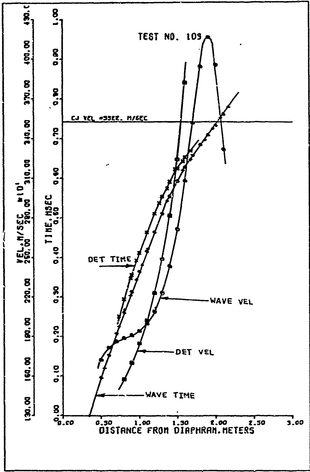
Figure 11. Plot of Data Obtained From Test 103, 35.40% Hydrogen, 14.94% Oxygen, and 49.66% Helium.
