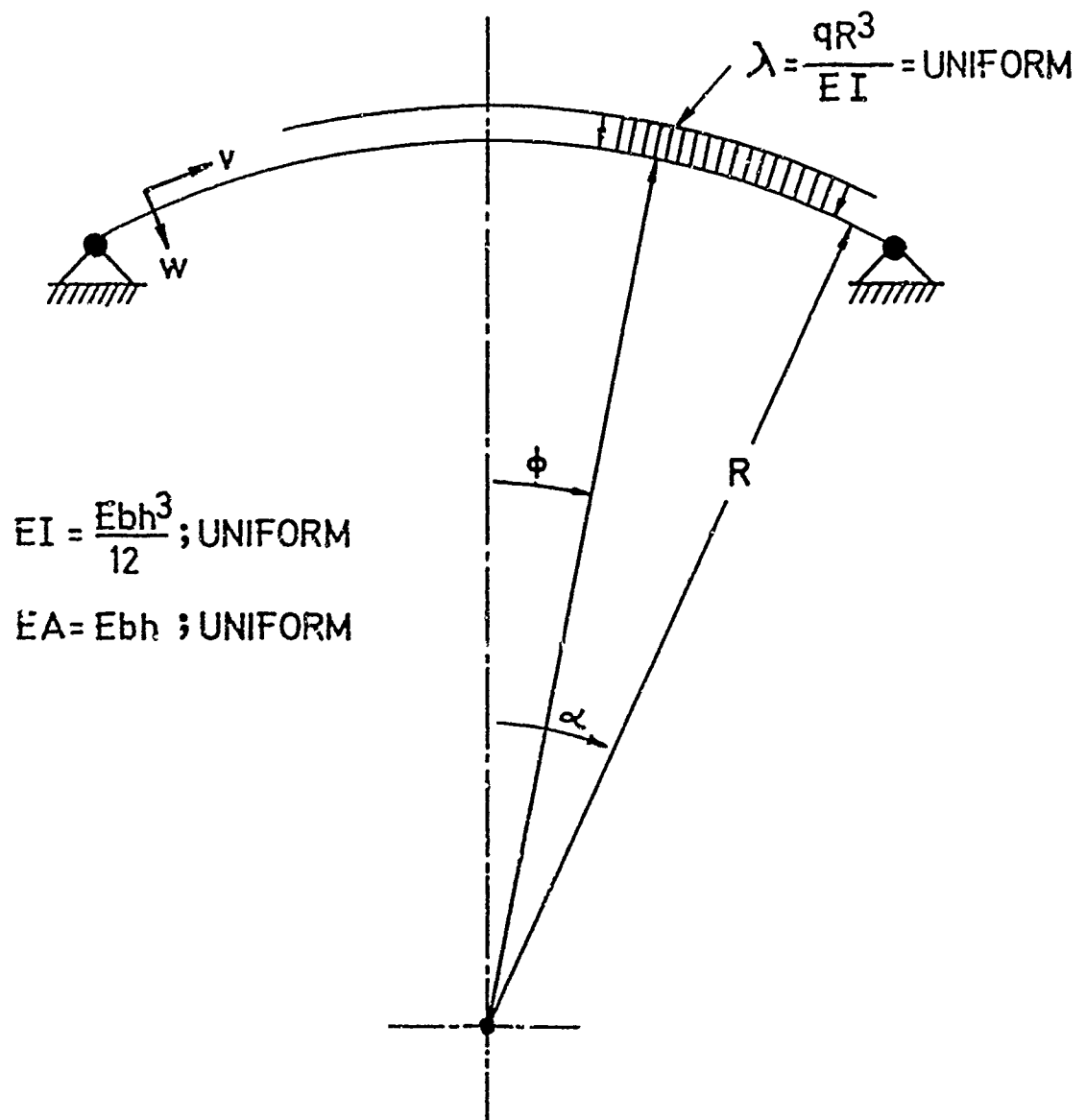
FIGURE. 1 ARCH GEOMETRY AND LOADING
