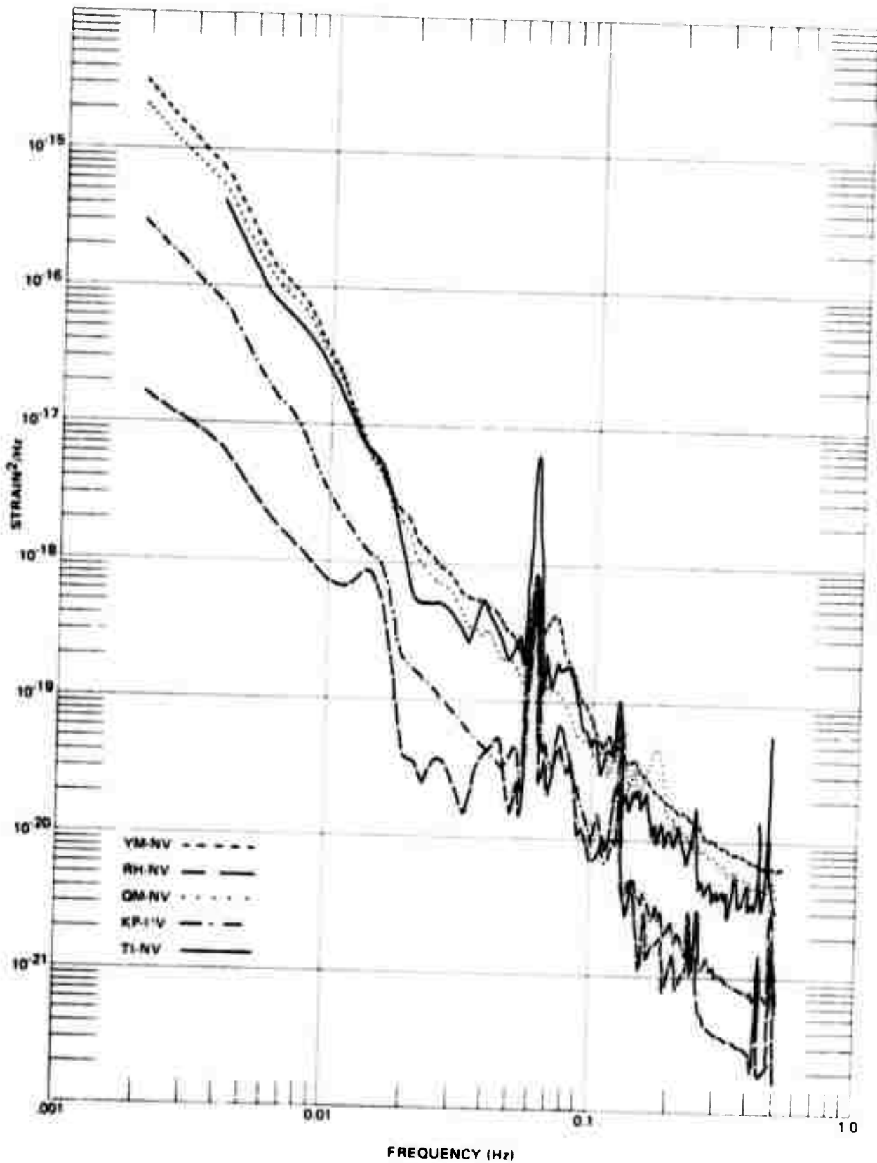
Figure 24. Power spectral density in \text{strain}^2/\text{Hz} of noise and signal for NTS event MINIATA recorded on the primary strain channel at 5 portable strain sites on 08 July 1971. The Nyquist frequency is 0.5 Hz.
