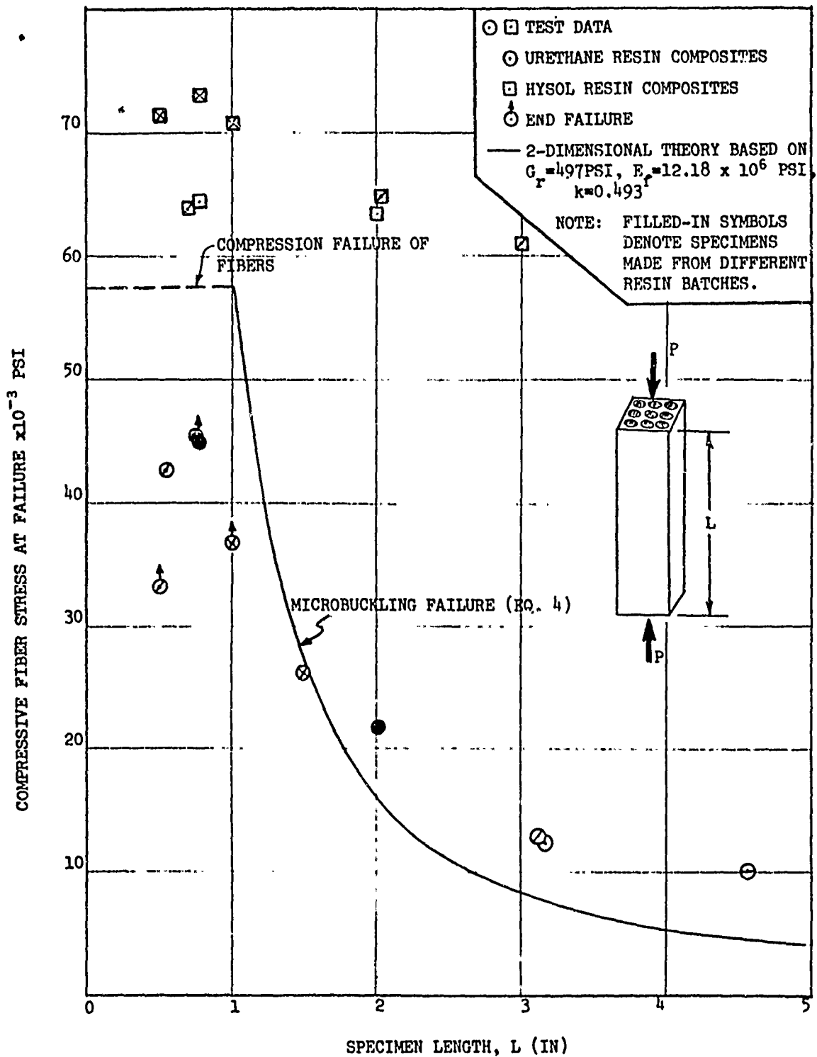
Figure 19. Test-Theory Correlation for Compressive Strength of Nine-Rod Composite Specimens
