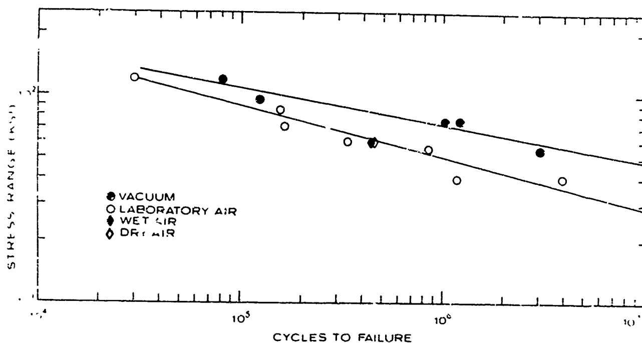
Fig. 13 Effect of vacuum on the fatigue life of nickel-base superalloy single crystals (after Duquette and Gell 12 ).
