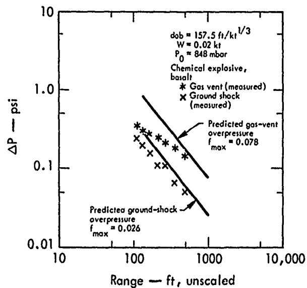
Fig. 23. Observed and predicted airblast overpressures for Buckboard 12.
