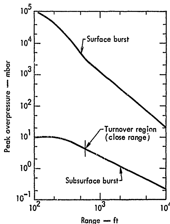
Fig. 2. Comparison of airblast overpressure as a function of range for 1.0-kt surface and subsurface detonations.
