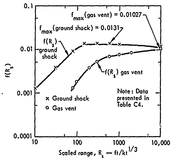
Fig. 12. Cabriolet ground-shock and gas-vent f-values as a function of R_s .
