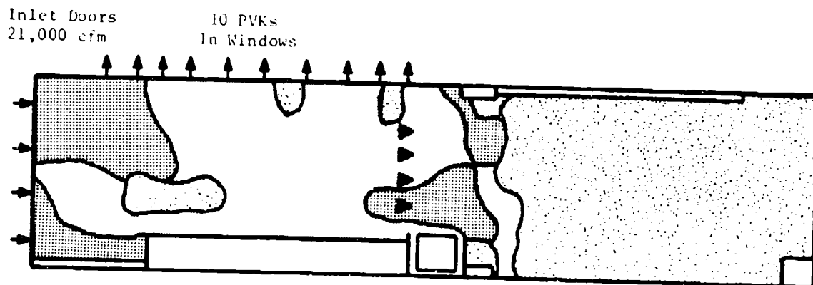
b. THREE-FOOT LEVEL CONTOURS.
