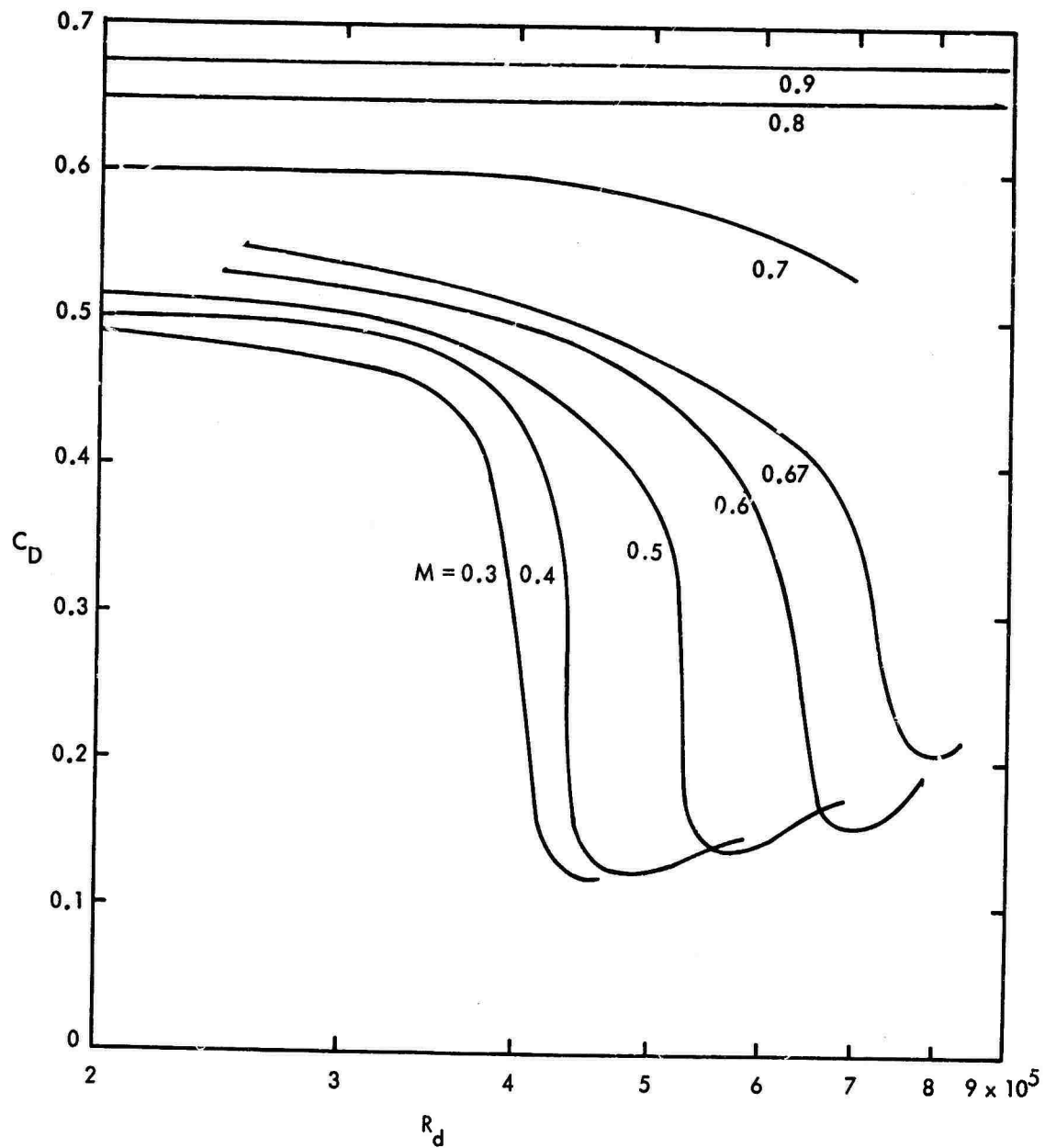
FIG. 8 DRAG COEFFICIENT OF SPHERES AS A FUNCTION OF REYNOLDS NUMBER AND MACH NUMBER IN THE REGION 2 \times 10^5 < R_d < 9 \times 10^5 , (NAUMANN, REF. (8) )
