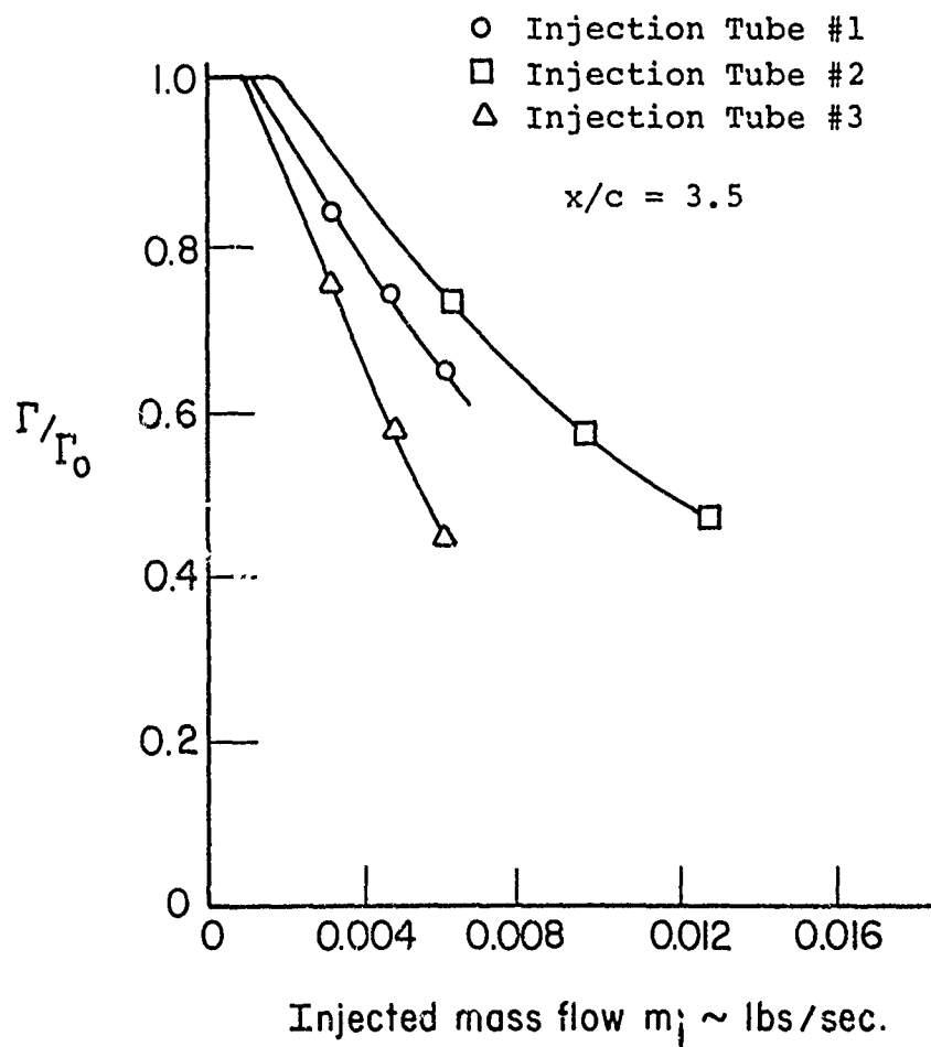
Figure 16. \Gamma/\Gamma_0 Versus Injected Mass Flow for Various Injection Tubes - V=115 ft/sec; \alpha=\pm 15^\circ (Split-Flap Vortex Generator).
