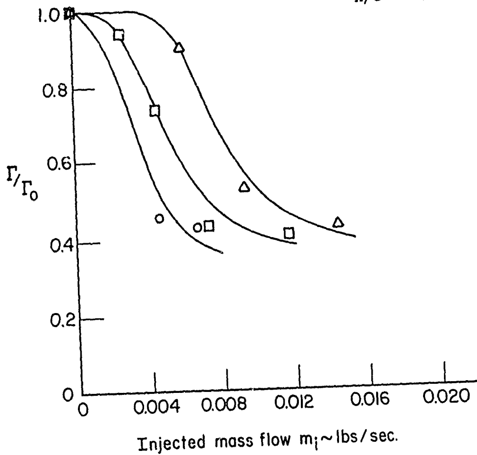
Figure 31. \Gamma/\Gamma_0 Versus Injected Mass Flow for Injection Tube Nozzles; V=75 ft/sec; \alpha=15^\circ .
