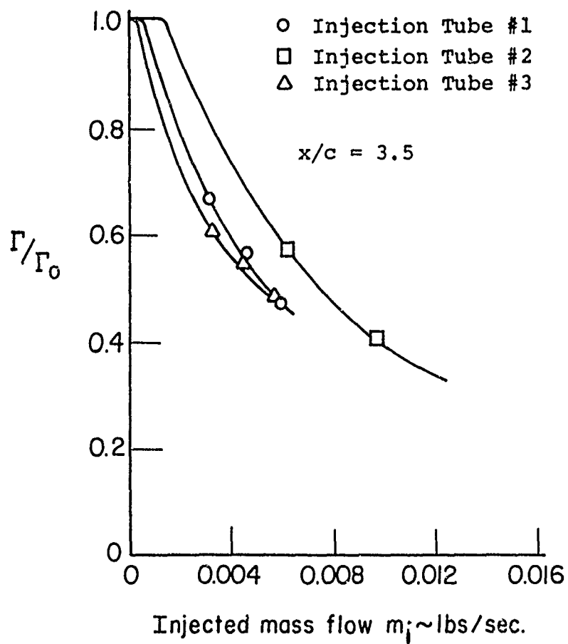
Figure 15. \Gamma/\Gamma_0 Versus Injected Mass Flow for Various Injection Tubes - V=75 ft/sec; \alpha=\pm 15^\circ (Split-Flap Vortex Generator).
