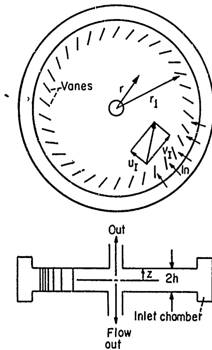
Figure 1. Typical Short-Vortex Chamber Configuration.
