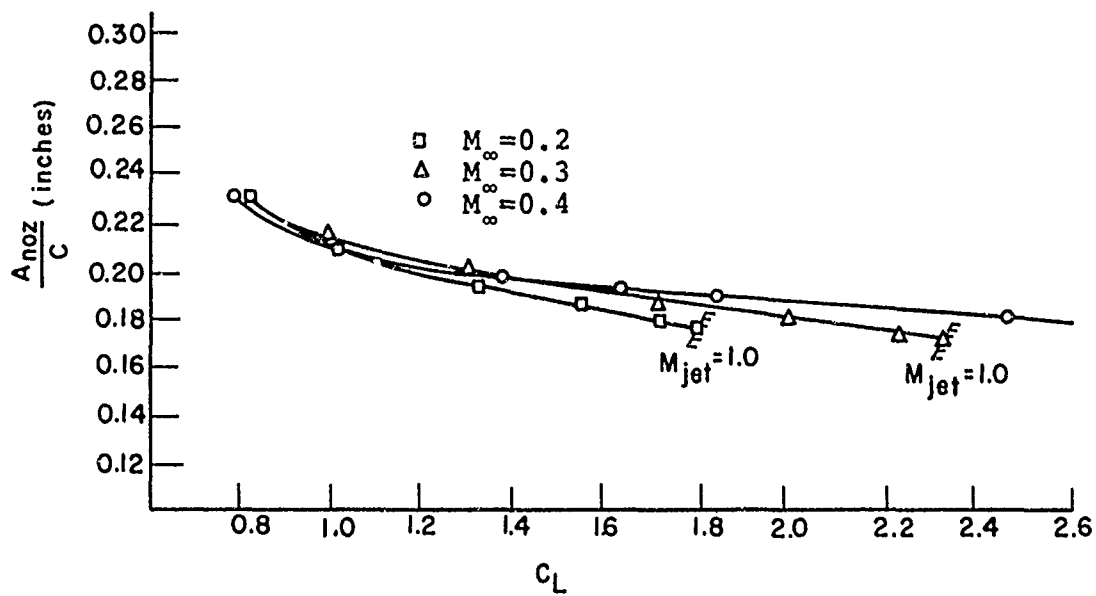
Figure 37. Minimum Nozzle Area for Tip Vortex Dissipation.
