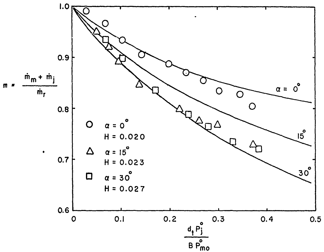
Figure 15. Net Throttling Available for Various Angles of Injection.
