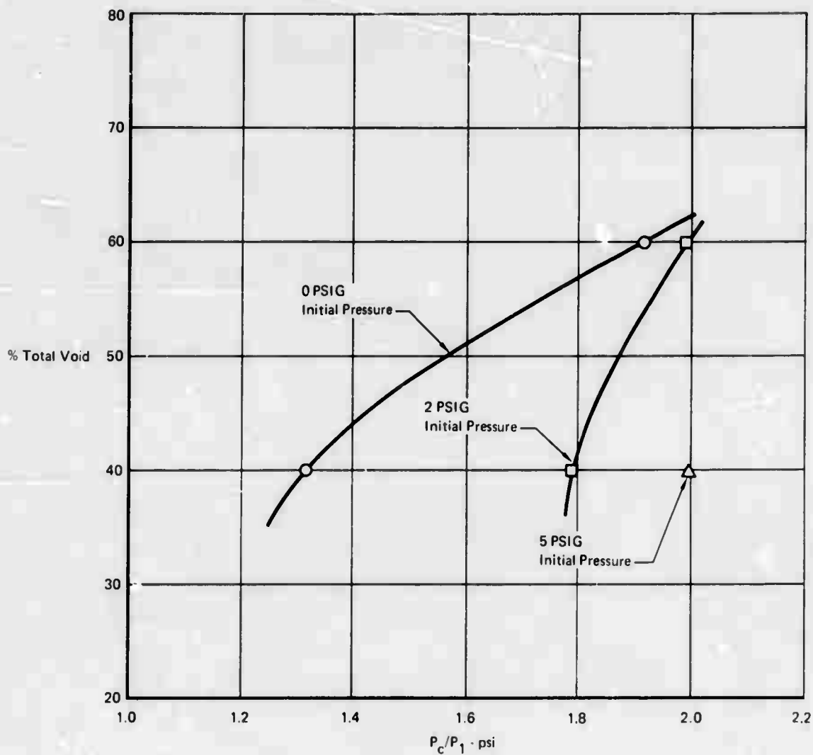
FIGURE 34 SIX CELL WING TANK CYLINDER TESTS 15 INCH DIAMETER
