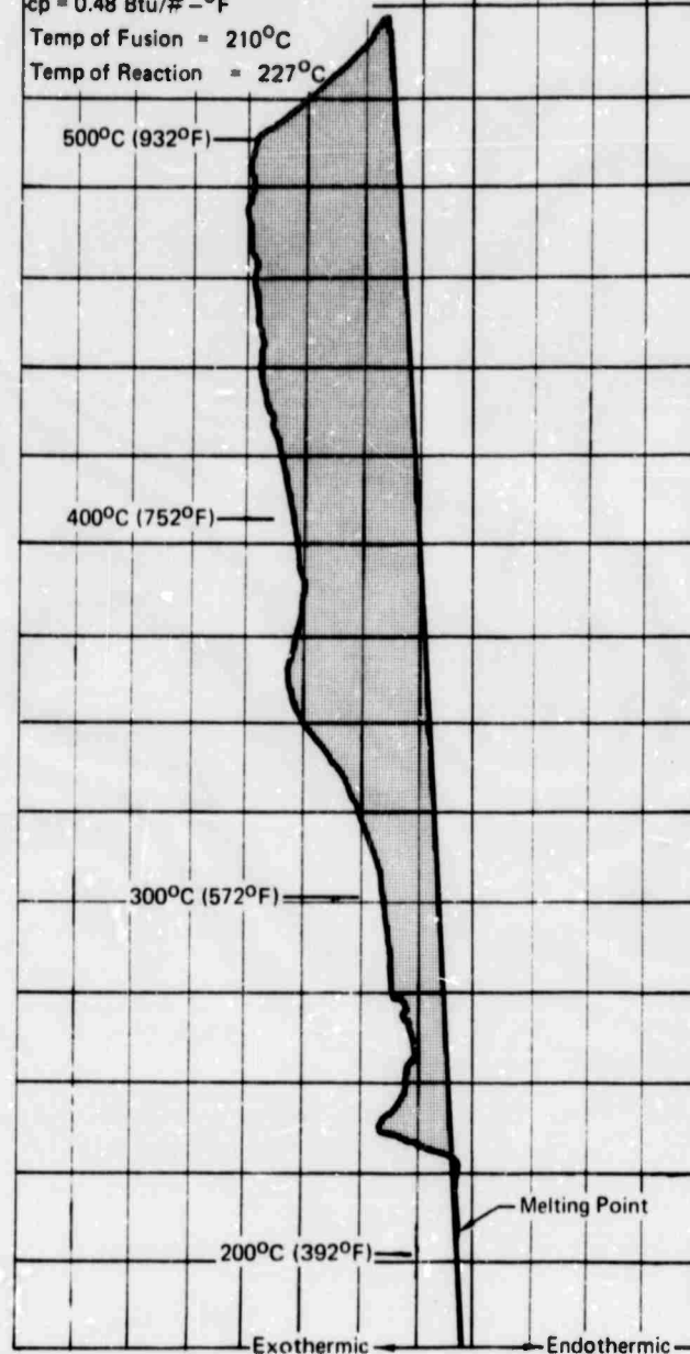
FIGURE 46 DTA TRACE
