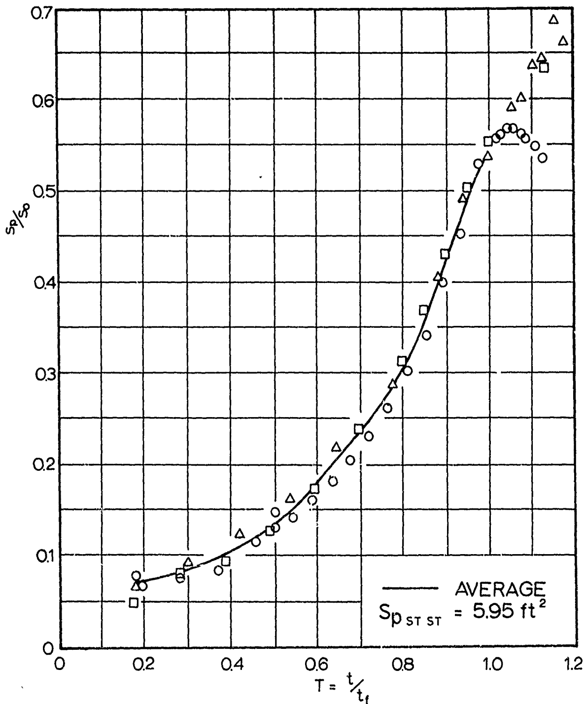
Fig 9 Area - Time History of a Model Ringslot Parachute, \eta = 0.40 , D_o = 3.77 \text{ ft} , m_i/m_s = 0.32 , V_s = 85 \text{ fps}
