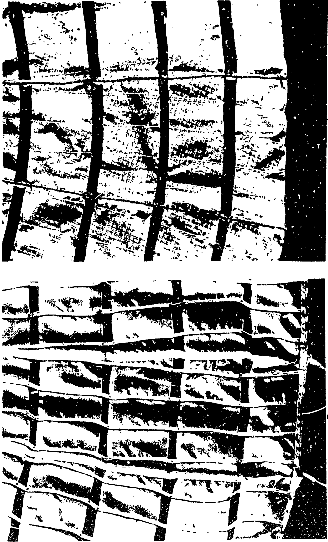
Fig 1 Fabrication Details of a Conventional, a, and a more Flexible, b, Ringslot Parachute Model
