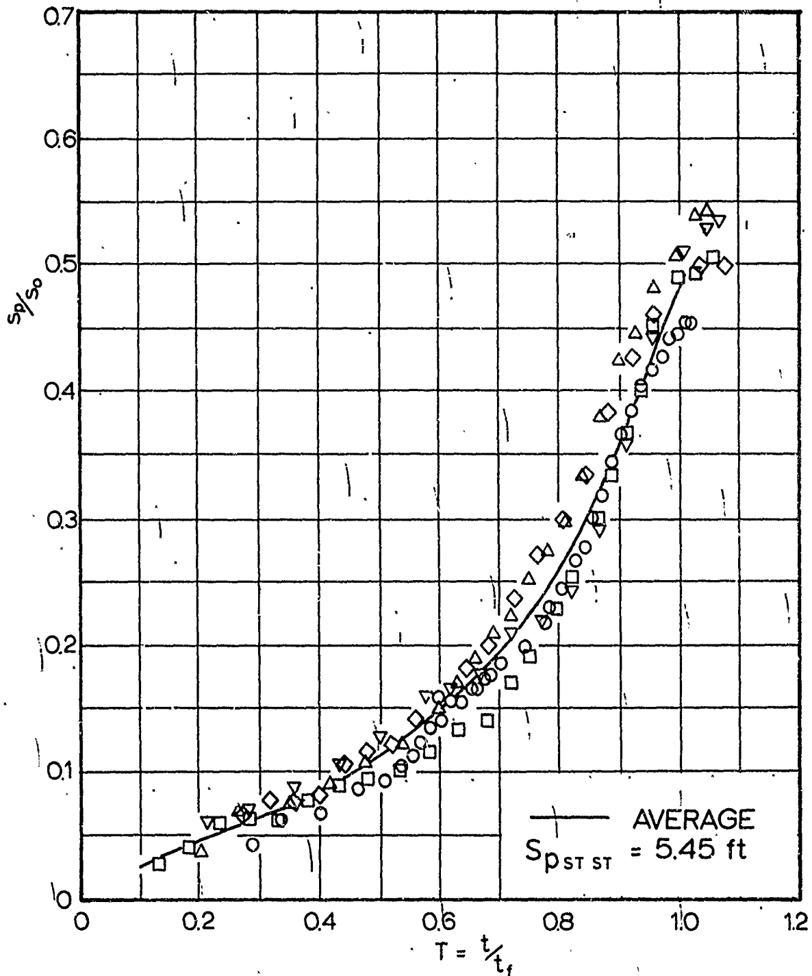
Fig 7 Area - Time History of a Model Ringslot Parachute, \eta = 0.40 , D_o = 3.77 \text{ ft} , m_i/m_s = 0.32 , V_s = 50 \text{ fps}
