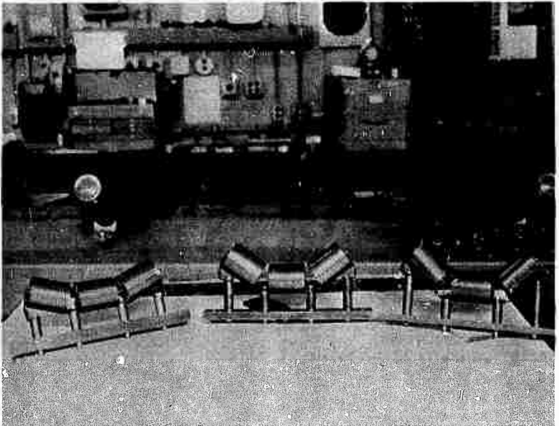
Fig. 3 Typical idler assemblies
