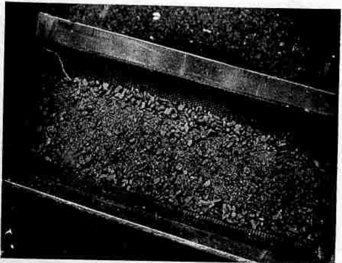
Fig. 6 Bulk material at angle of repose prior to testing
