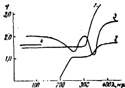
Figure 3. Spectral curves of contrast coefficient of films: 1 -- UF-2T; 2 -- UFSh-0; 3 -- UF-1L; 4 -- UF-αt.
