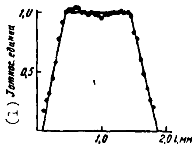
Figure 1. Illumination distribution of mercury line 334 \mu by height. KEY: 1. Relative units.
