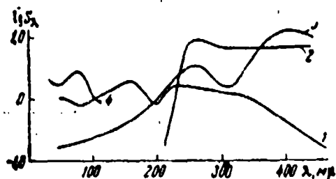
Figure 2. Spectral sensitivity curves of films: 1 -- UF-2T; 2 -- UFSh-0; 3 -- UF-1L; 4 -- UF-αt.
