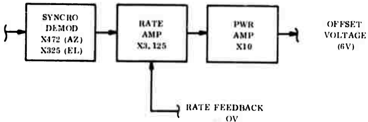
Figure 8-26. Static Offset
