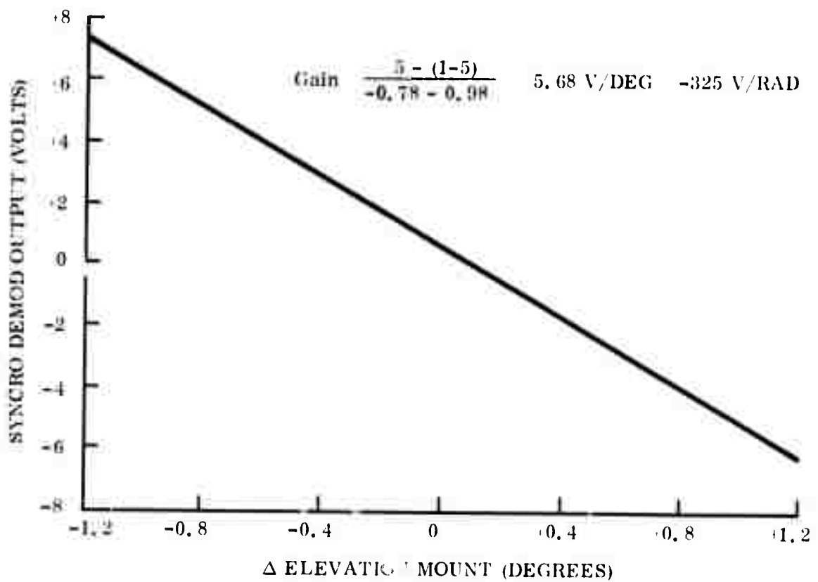
Figure 8-11. Azimuth and Elevation Position Gain Calculation
