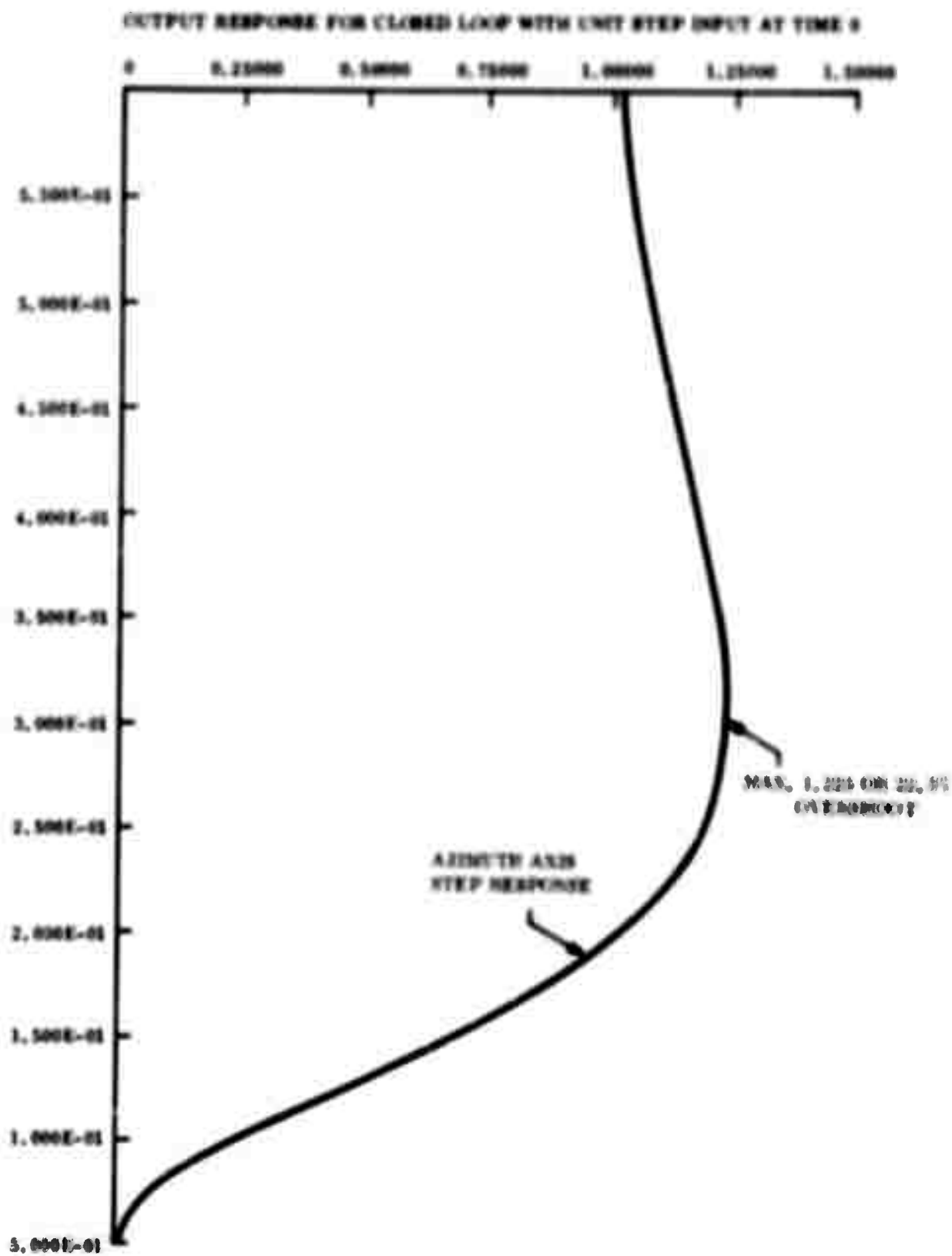
Figure 4-22. Azimuth Position Loop Step Response (Corrected for Motor Plus Load Inertia)
