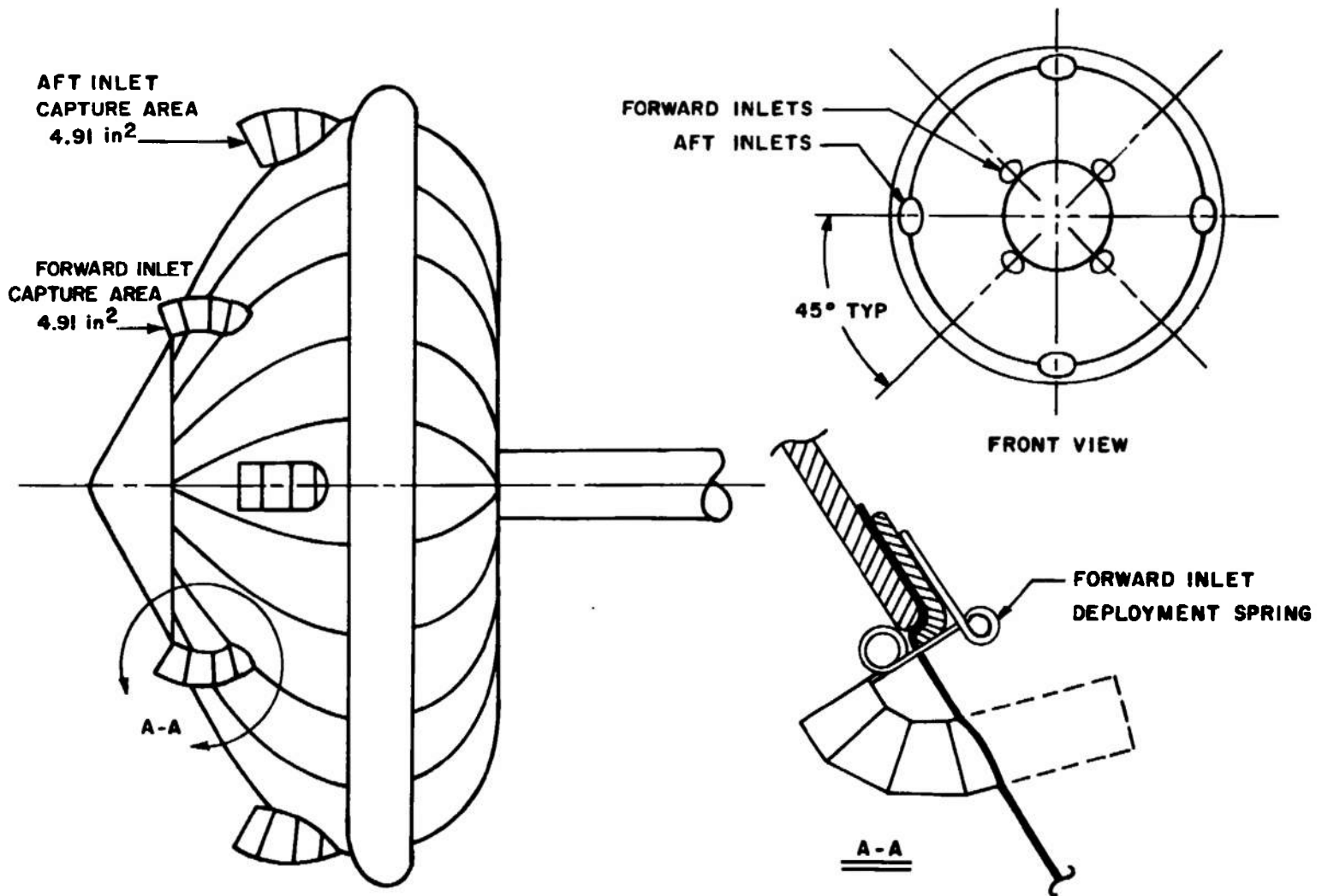
Fig. 4 Inlet Location
