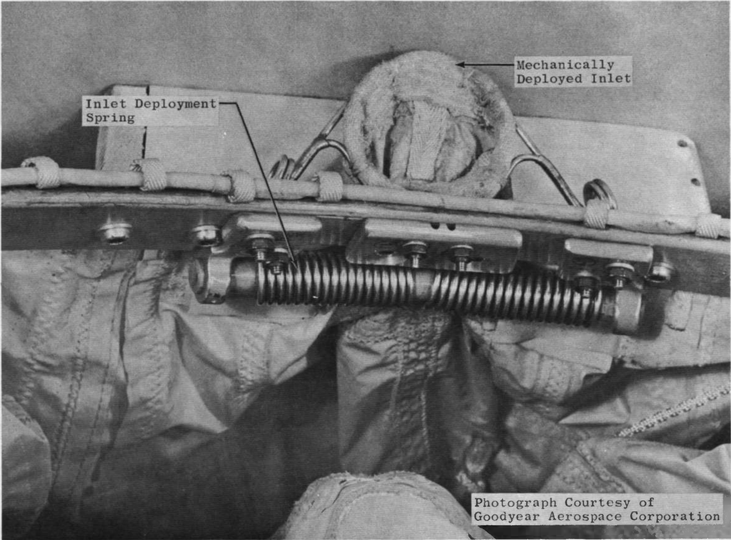
Fig. 2 Inlet Deployment Spring
