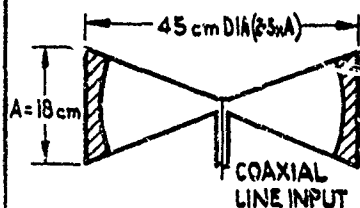
FIG. 1b LENS CORRECTED BICONICAL HORN
