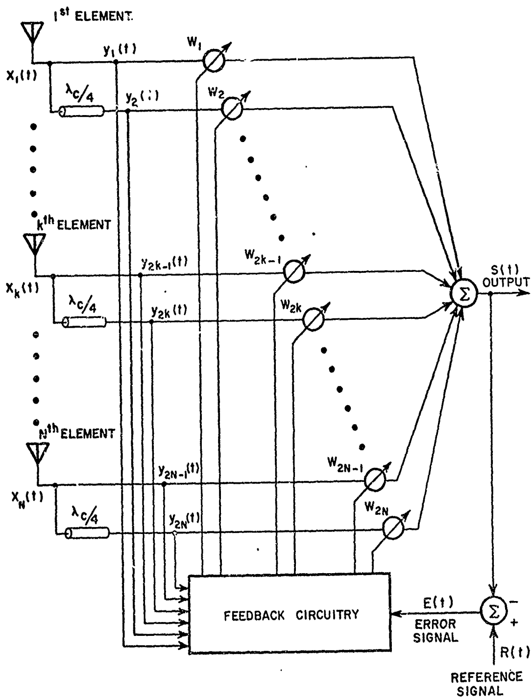
Fig. 1. The basic adaptive array.
