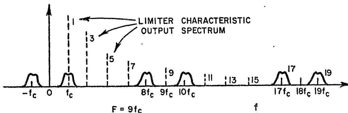
Fig. 12. Second digital filter input spectrum and periodic frequency response characteristics.
