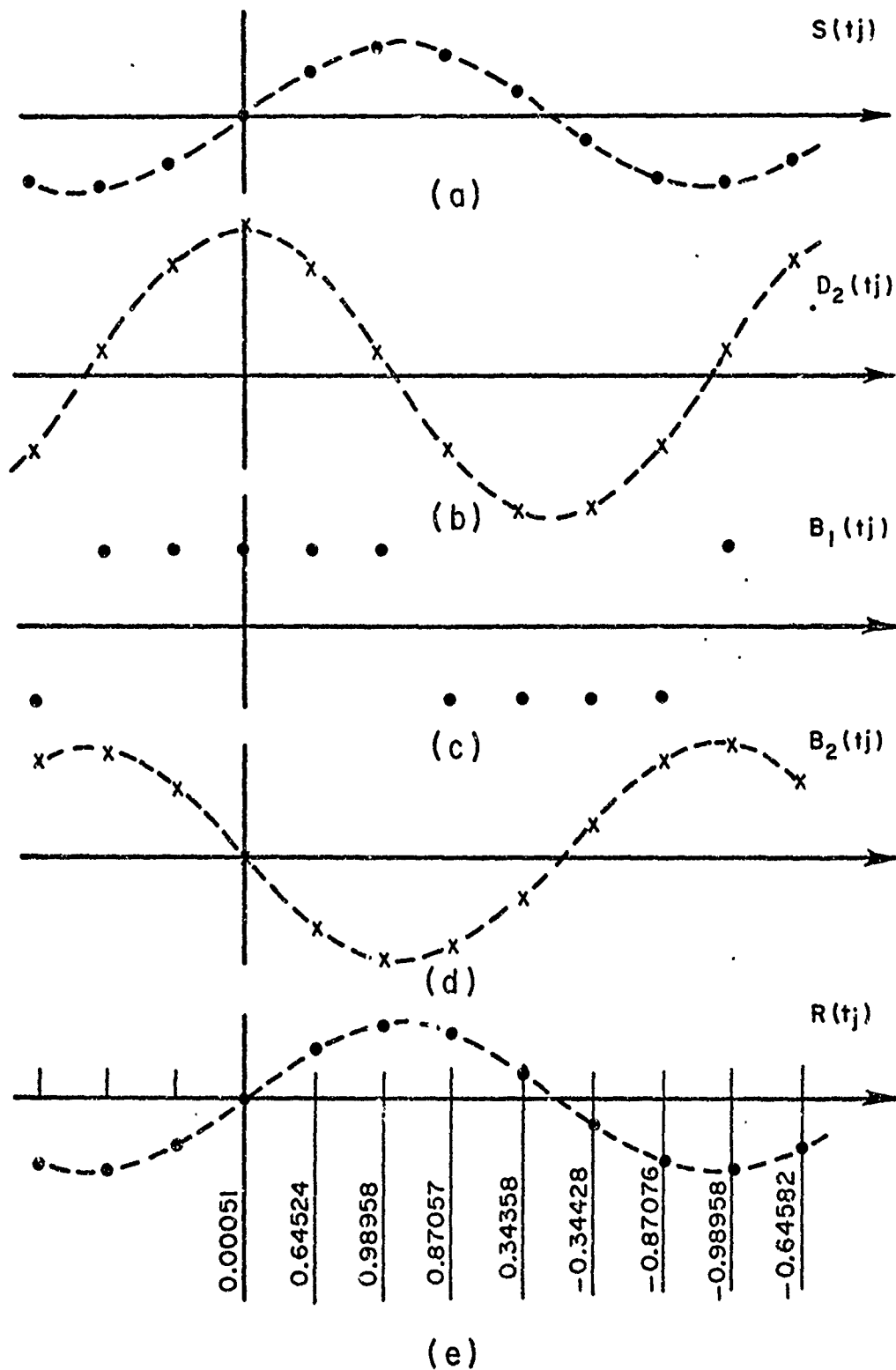
Fig. 13. Reference network sampled-data waveforms.
