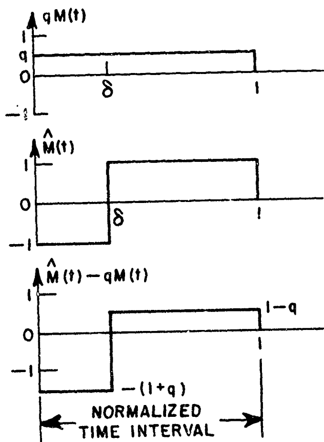
Fig. 33. Example waveforms for calculating mean-square error.
