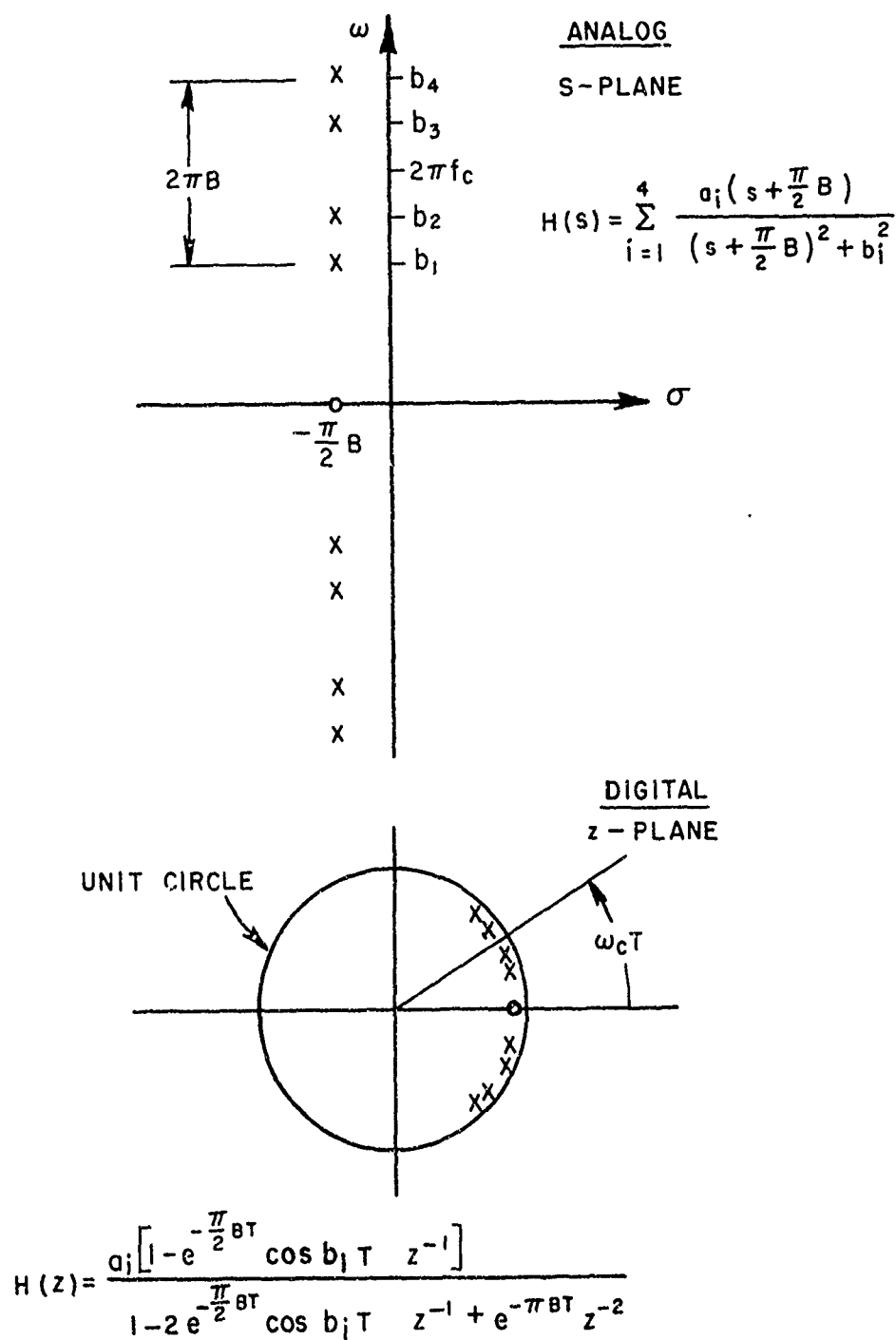
Fig. 7. Pole-zero configuration of 4th order Lerner filter.
