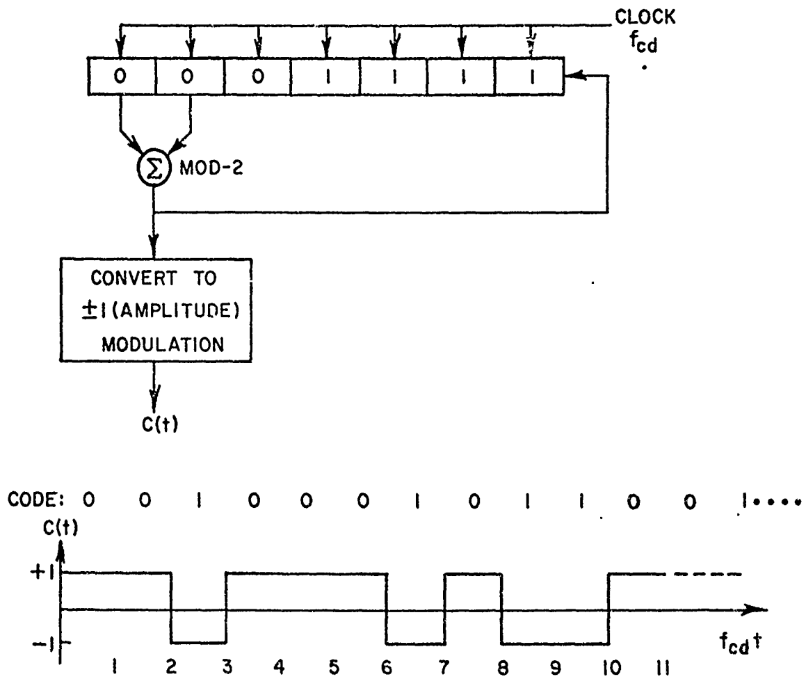
Fig. 5. Pseudorandom code modulation generation.
