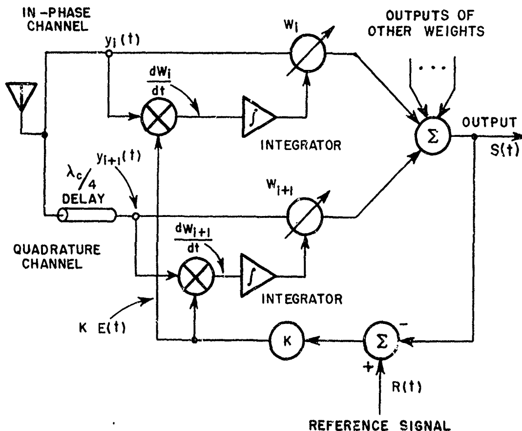
Fig. 2. Feedback circuitry for each element of the array.
