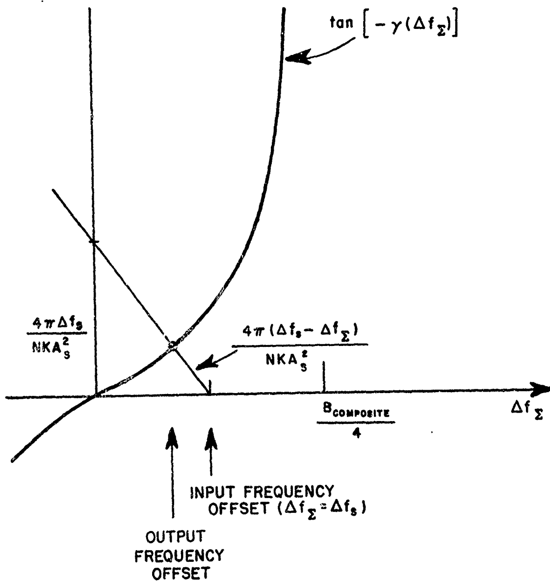
Fig. 20. Results of desired signal frequency offset analysis.
