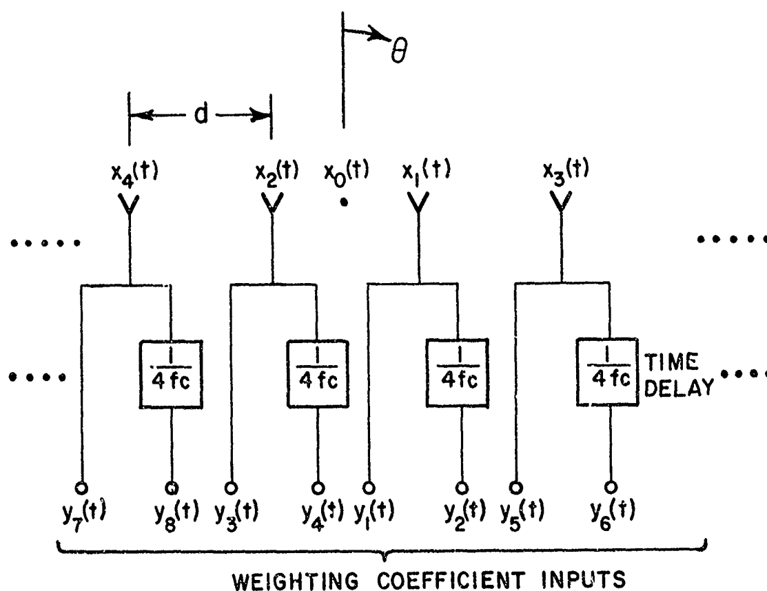
Fig. 4. Linear array geometry.
