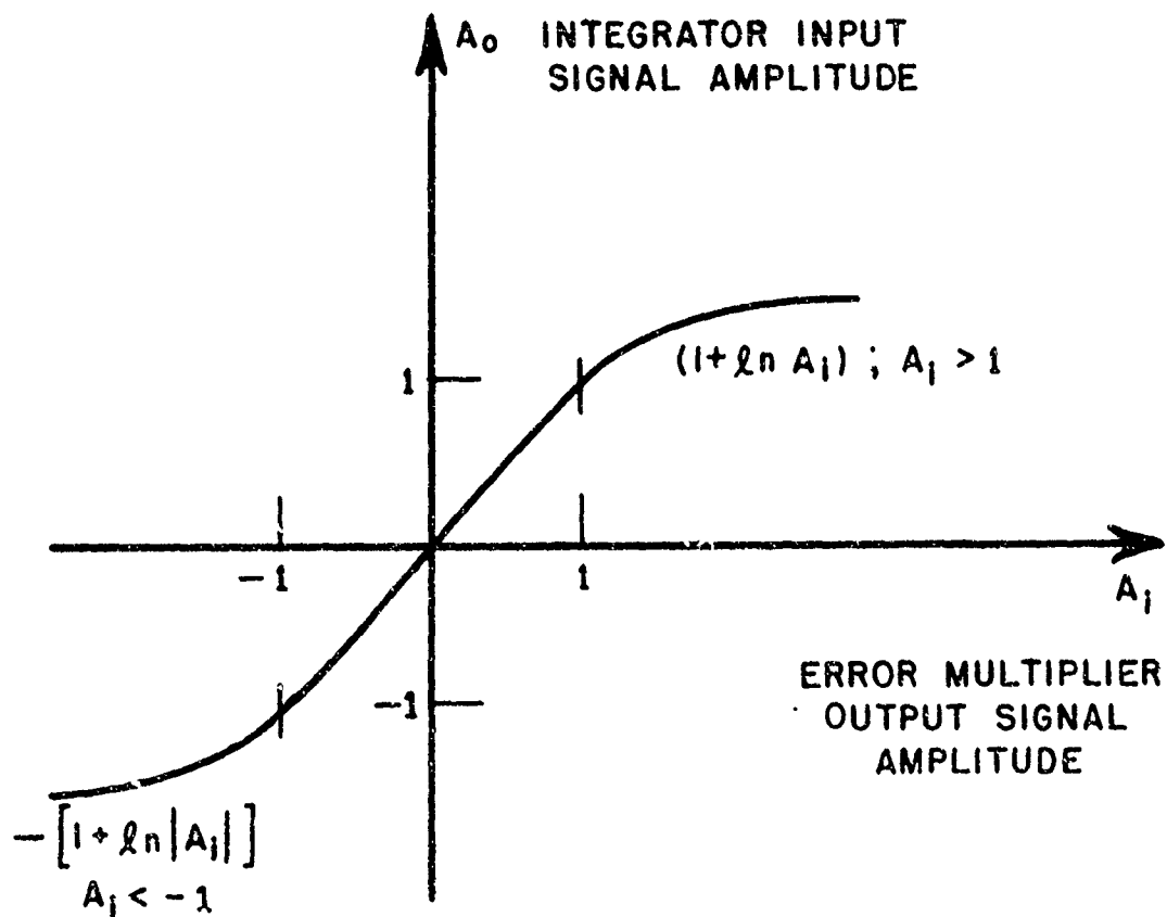
Fig. 31. Simulation characteristic for error multiplier output amplitude saturation.
