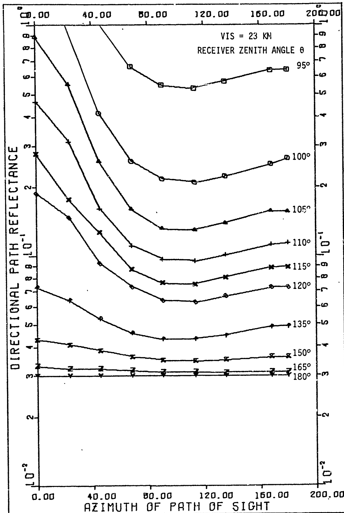
Fig. 46. Directional Path Reflectance Versus Azimuth for a Solar Zenith Angle of 78^\circ . The Albedo is .06, Wavelength is .55 \mu\text{m} , and the Altitude is 2 KM. Data from AWS Model.
