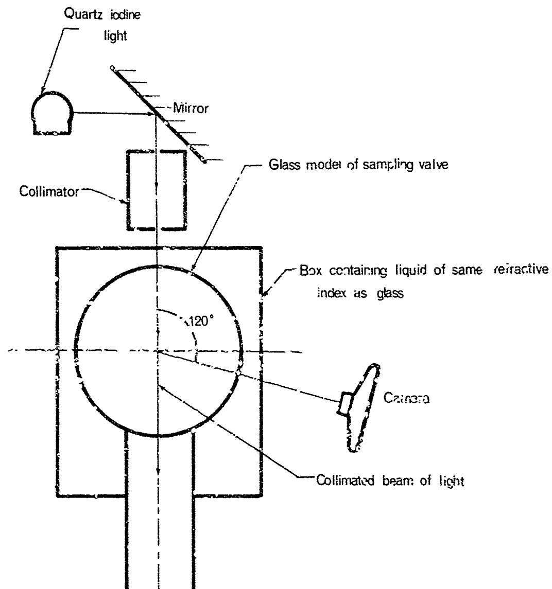
FIGURE 10 Apparatus for flow visualisation
