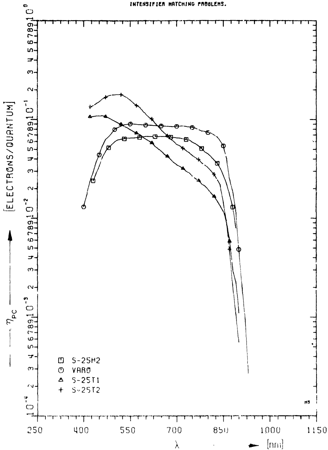
FIG. 8. SPECTRAL EFFICIENCIES, \eta_{PC} , OF PHOTOCATHODES
