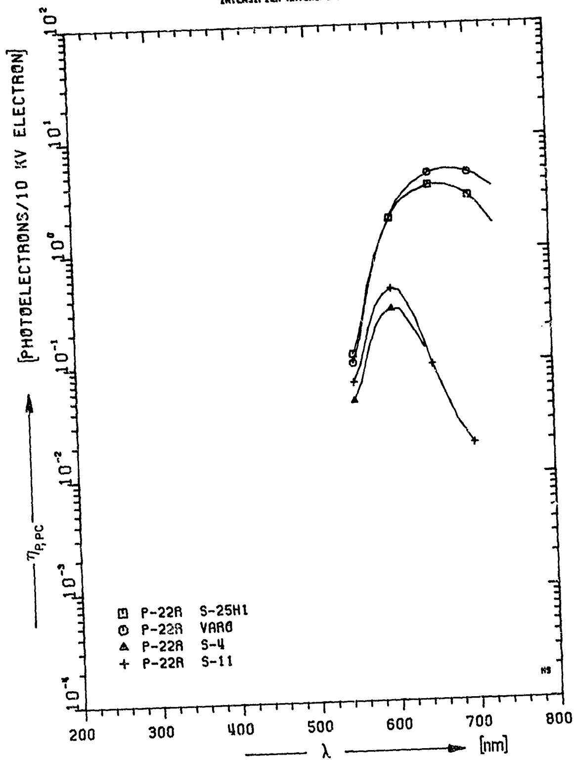
FIG.20B. SPECTRAL RESPONSE, \eta_{P,PC} , OF PHOSPHOR SCREEN - PHOTOCATHODE COMBINATIONS.
