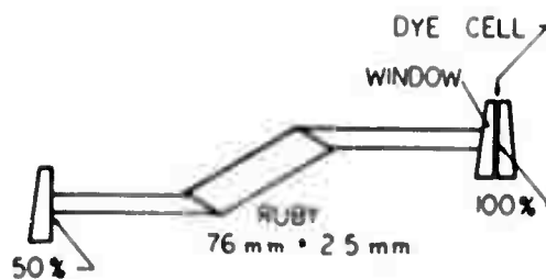
Figure 9. Oscillator Cavity
