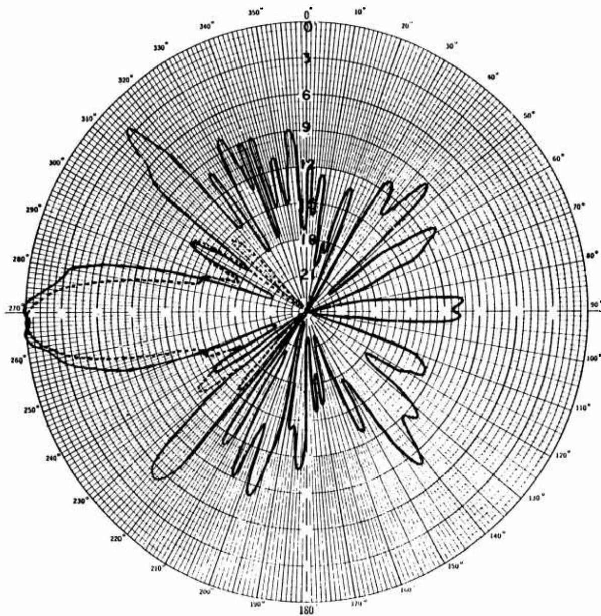
Figure III-9 WEST RHOMBIC HORIZONTAL POLARIZATION Elevation 18°
