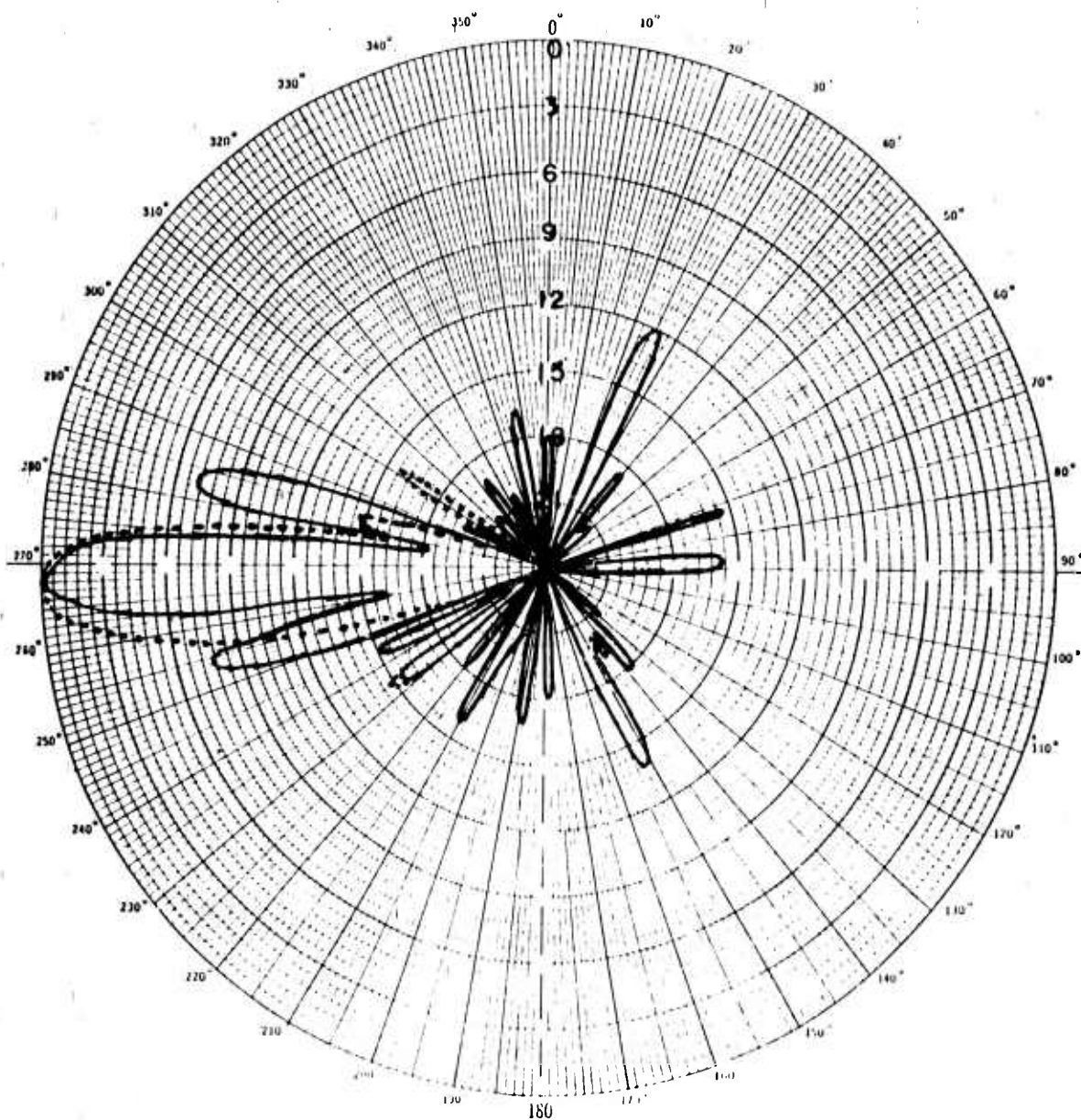
Figure III-18 WEST RHOMBIC HORIZONTAL POLARIZATION
