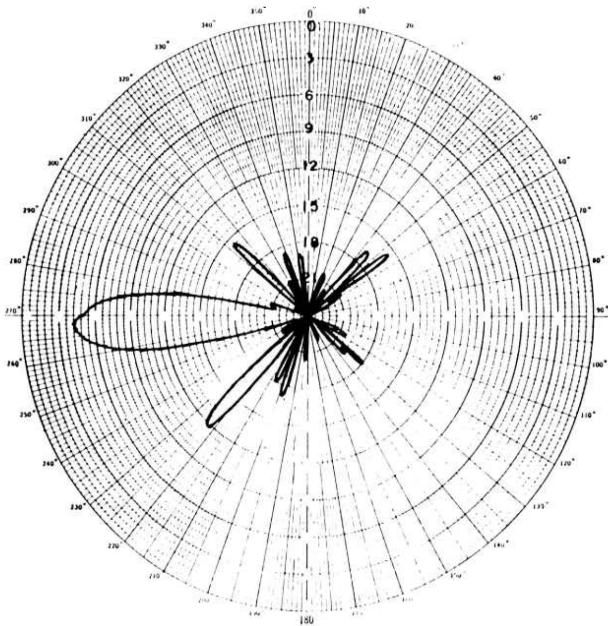
Figure III-3A WEST RHOMBIC HORIZONTAL POLARIZATION Frequency - 10.5 MHz Elevation 4°
