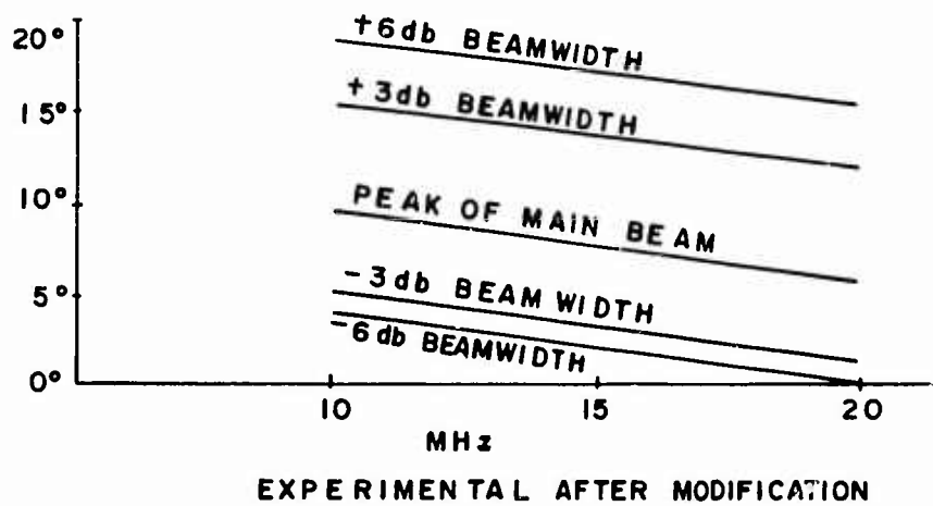
VERTICAL-PROFILE: BEAMWIDTH VS FREQUENCY
