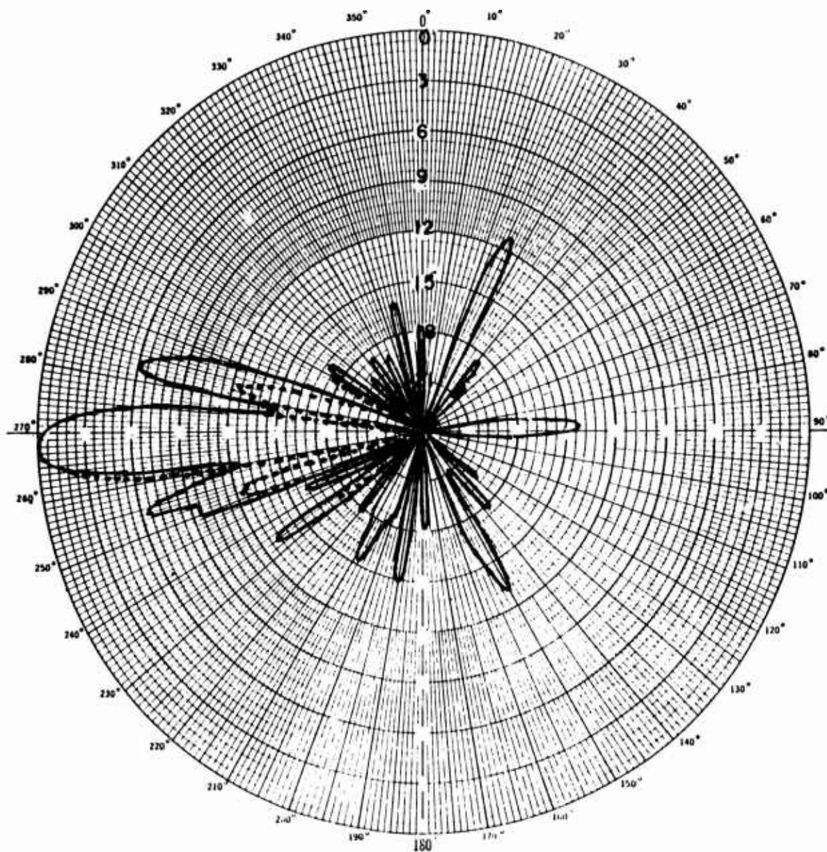
Figure III-19 WEST RHOMBIC HORIZONTAL POLARIZATION Elevation 22°
