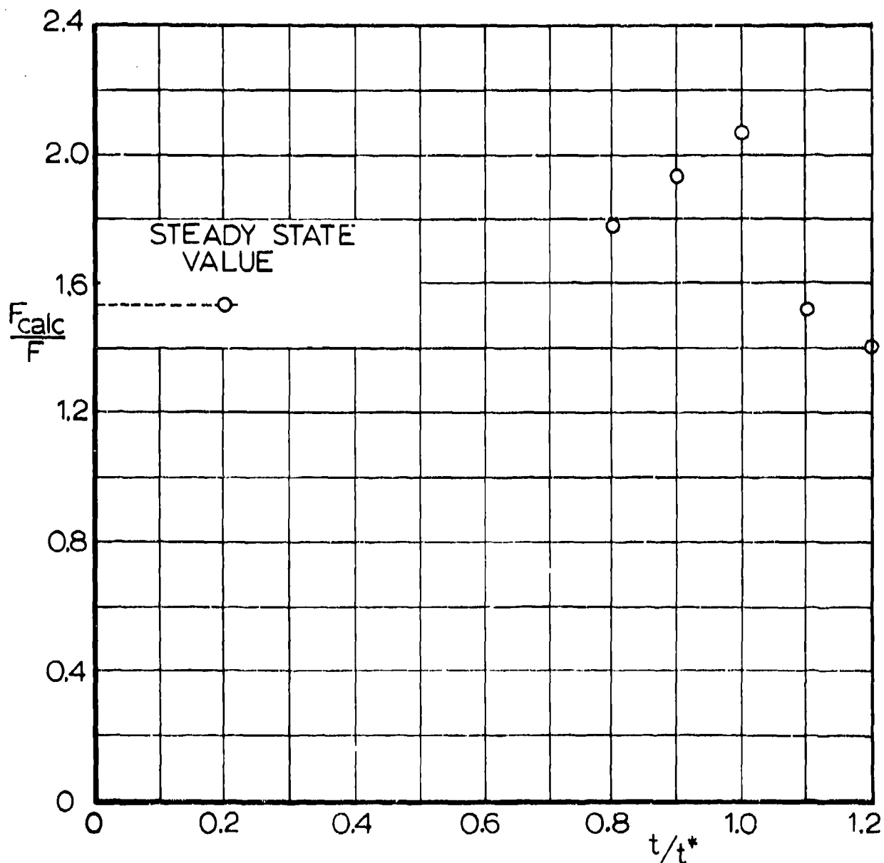
Fig 5 Ratio of Calculated and Measured Instantaneous Forces; Solid Flat Circular Parachute, V_0 = 70 ft/sec (Based on Refs 1, 2, Run 182)
