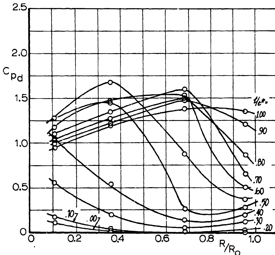
Fig 31 Measured Differential Pressure Coefficient vs Location; Ringslot Parachute, V_0 = 160 ft sec (Based on Ref 1, Run 18)
