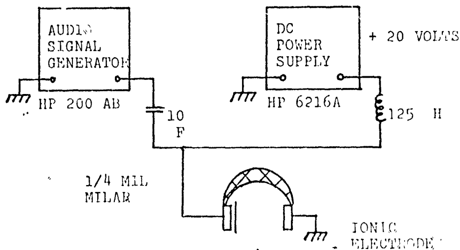
Figure 9. Electrophonic Effect with Low Power Mode
