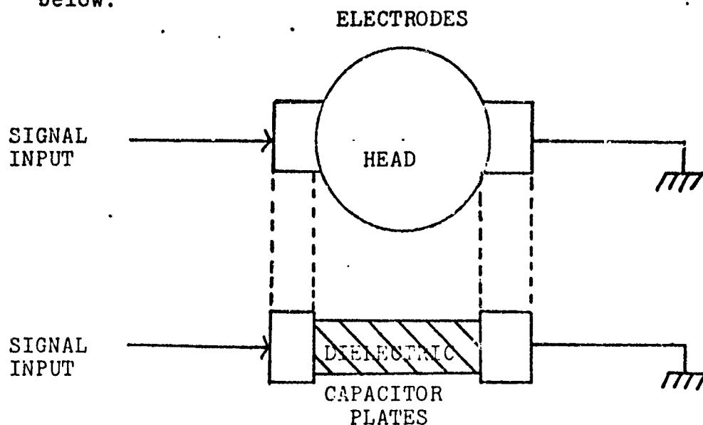
Figure 12. Capacitor Analog Using Pair of Capacitive Electrodes
