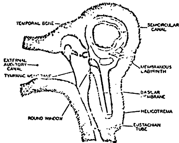
Figure 6. Inner Ear with Unspiralled Cochlea
