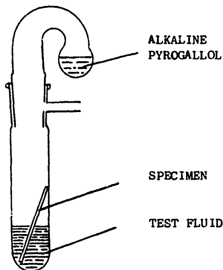
Fig.II : THUNBERG TUBE ASSEMBLY.
