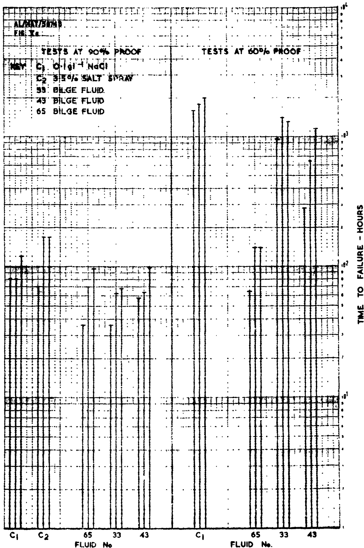
FIG. 5a STRESS CORROSION TESTS - VAAS. 554 SPECIMENS
