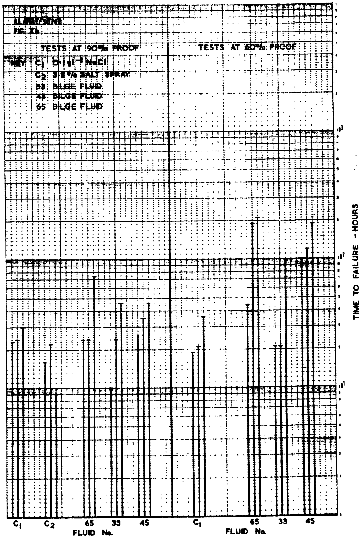
FIG. Vb STRESS CORROSION TESTS - DTD. 5050 SPECIMENS
