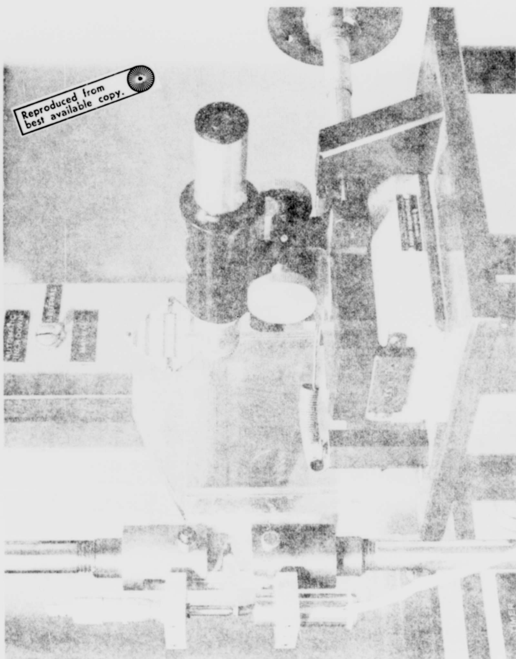
Fig. 2. Typical Experimental Test Setup Showing LVDT Measuring Changes in COD and Optical Traveling Microscope for Measuring Crack Length
