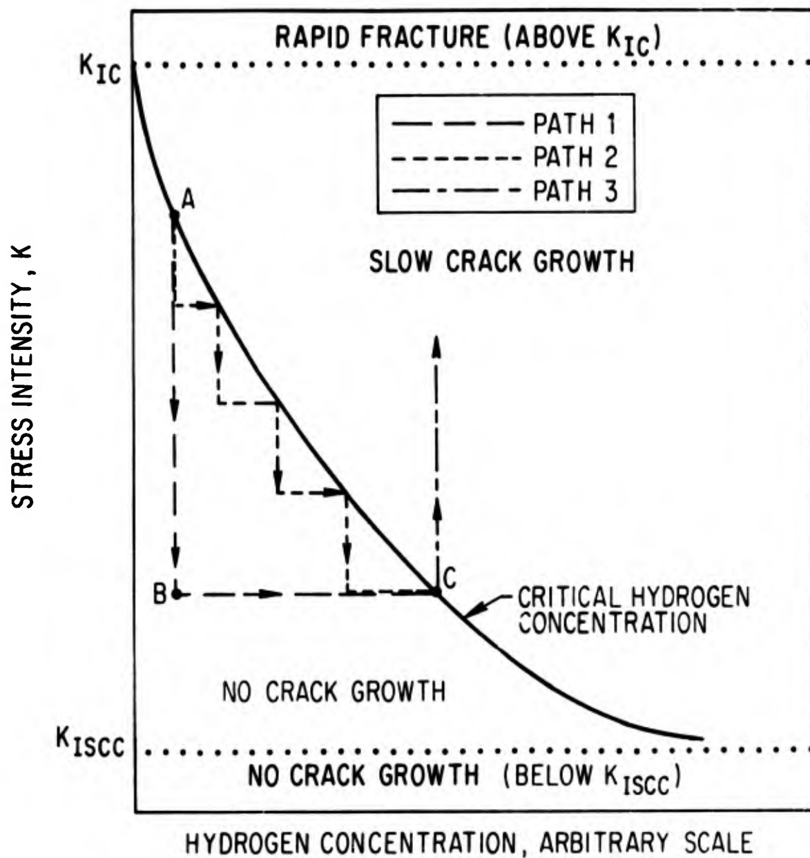
Fig. 7. Proposed Inverse Relationship Between Stress Intensity and Critical Hydrogen Concentration Required for Crack Growth
