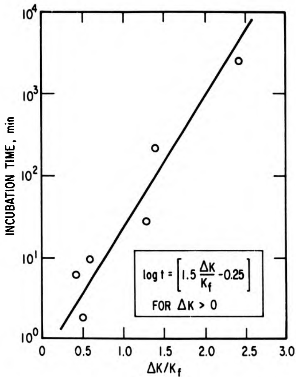
Fig. 5. Effect of Stress Corrosion Cracking History on Incubation Time for E-4340 HR Steel
