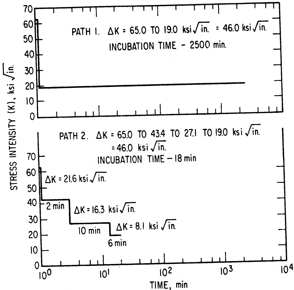
Fig. 4. Incubation Time by Two Different Paths for E-4340 HR Steel
