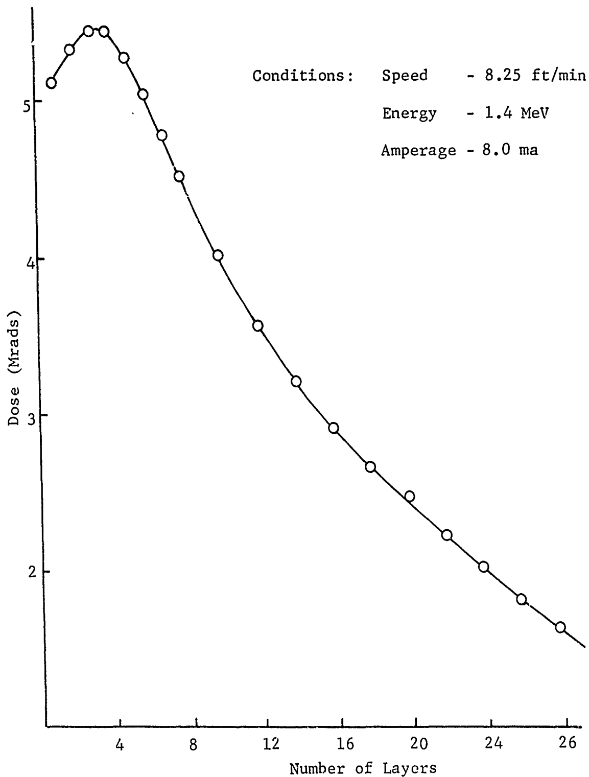
Figure 3-6 Dose Layer Curve for Arrangement of 2 Mil Film Spaced 1 Inch Apart Passing an Electron Beam
