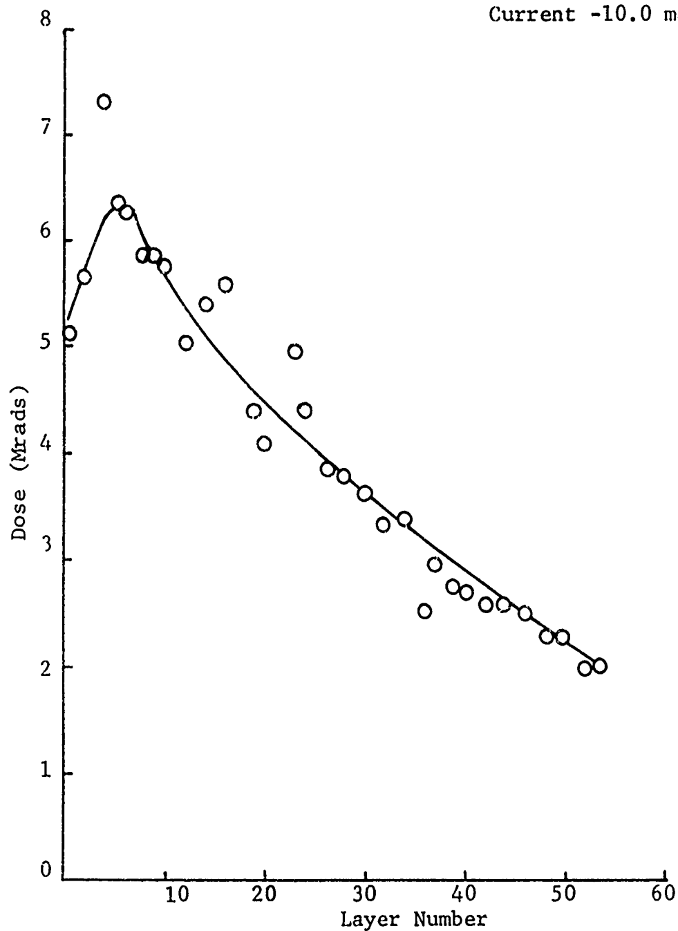
Figure 3-21 Dose Layer Curve for Arrangement of 1 Mil Film Spaced 0.8 Inch Apart Passing an Electron Beam.
