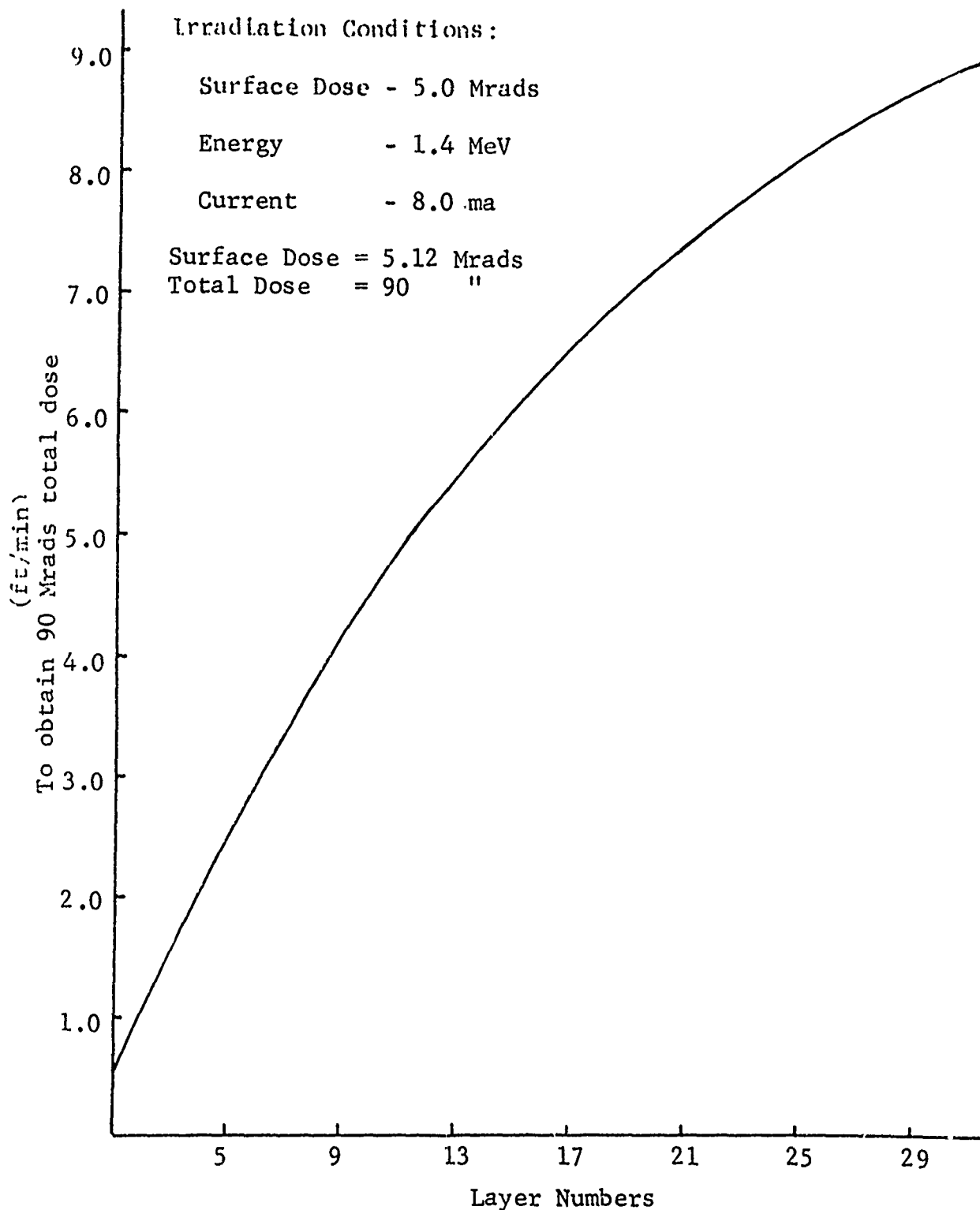
Figure 3-10 Film Velocity vs Number of Layers to Obtain 90 Mrads Total Dose For 3 Mil Film Spaced 1 Inch Apart
