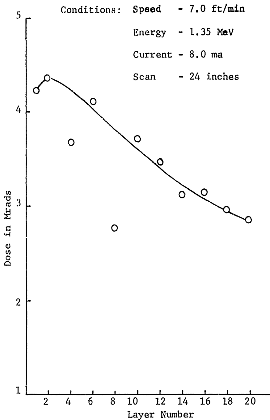
Figure 3-18 Dose-Layer Curve For 20 Layers of Two Mil Film.
