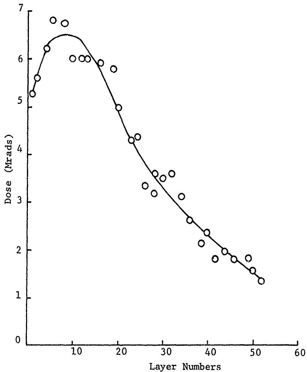
Figure 3-23. Dose Layer Curve for Arrangement of 3 Mil Film Spaced 0.8 Inch Apart Passing an Electron Beam.
