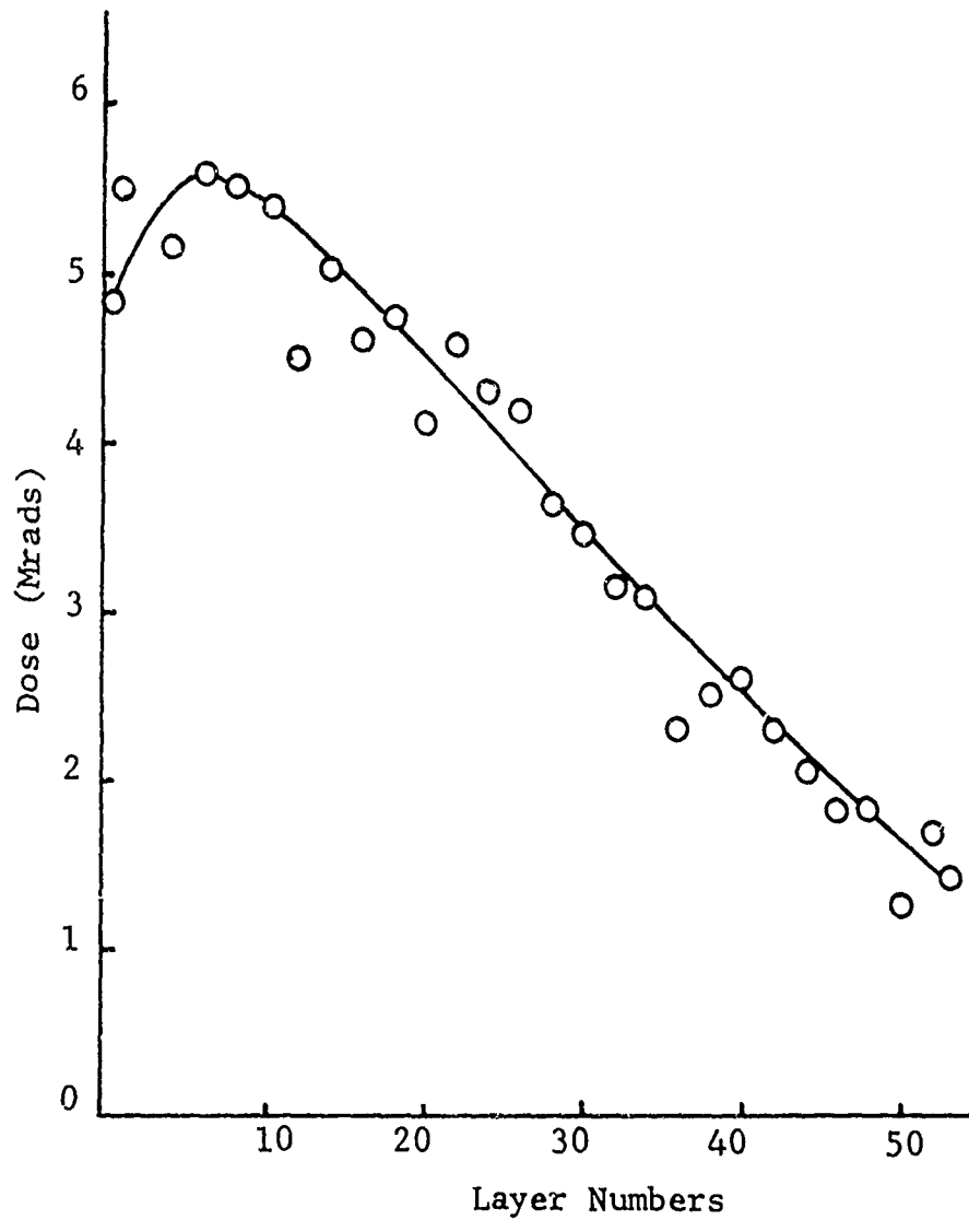
Figure 3-22. Dose Layer Curve for Arrangement of 2 Mil Film Spaced 0.8 Inch Apart Passing an Electron Beam.
