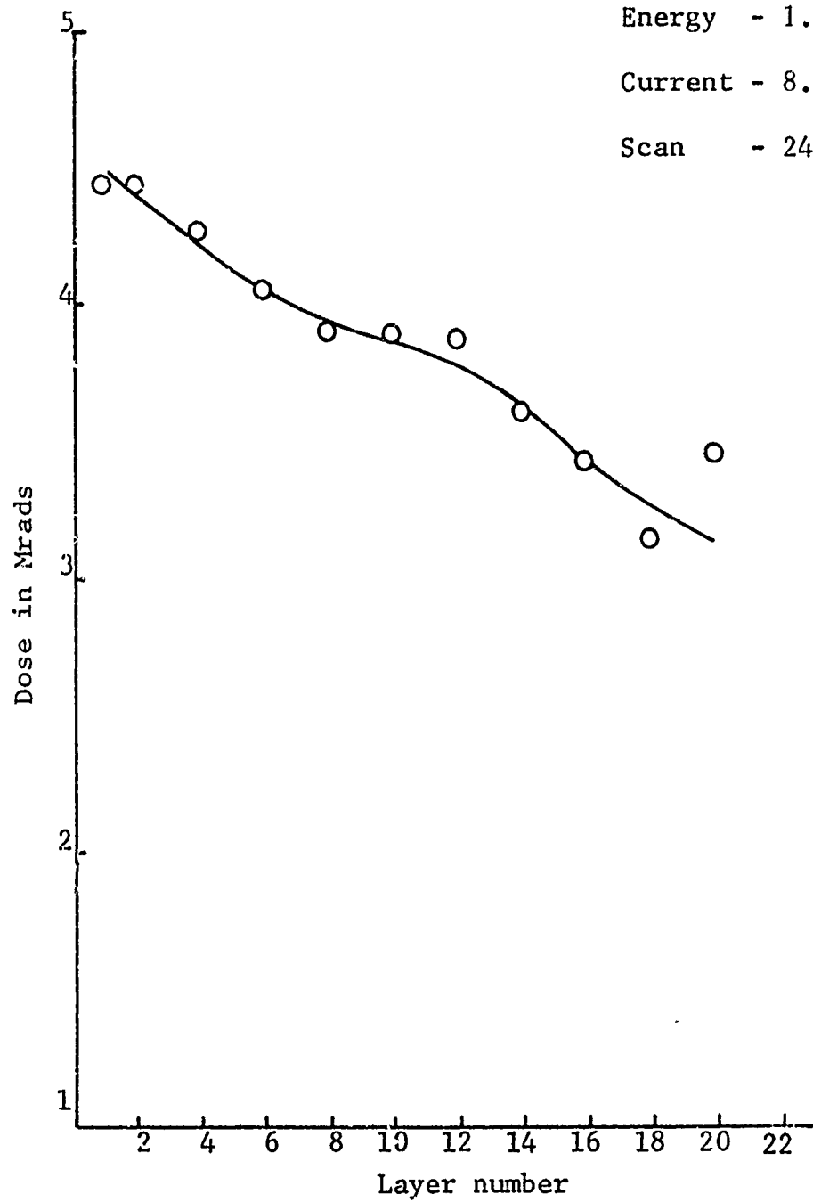
Figure 3-17 Dose-Layer Curve For 20 Layers of One Mil Film
