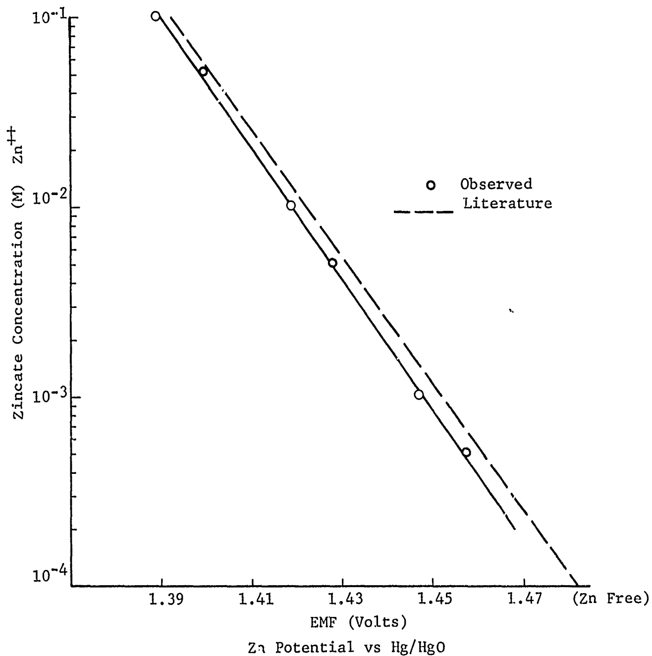
Figure 8-24. Calibration Curve for Zn Concentration and Potential in 45% KOH.
