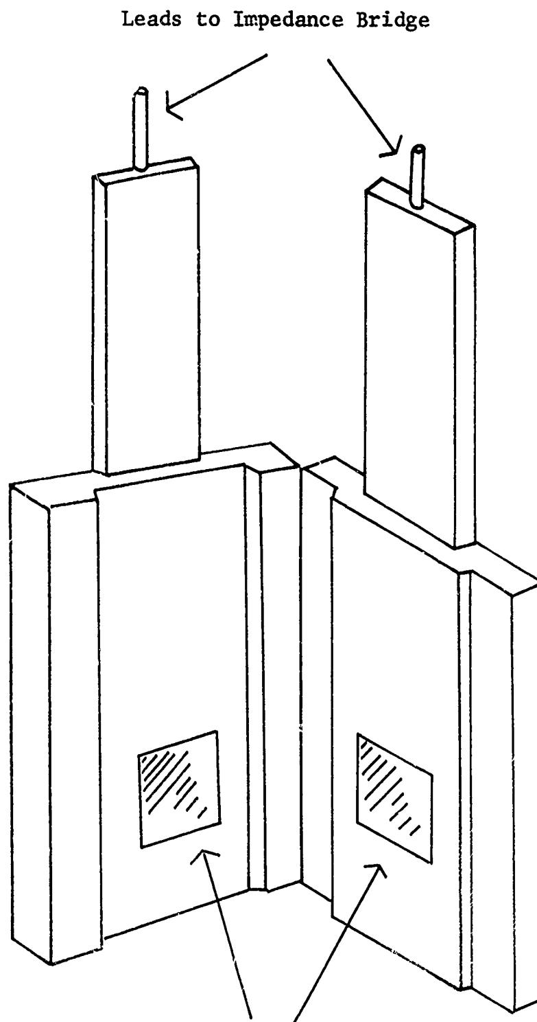
Platinized Platinum Electrodes
