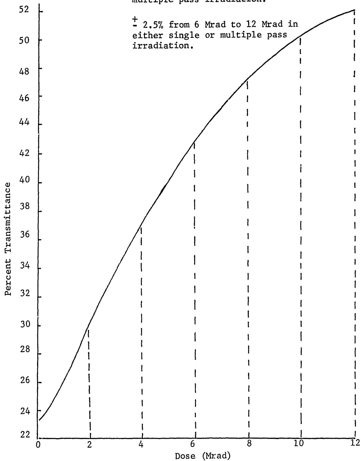
Figure 3-16 Dosimetry Calibration Curve
