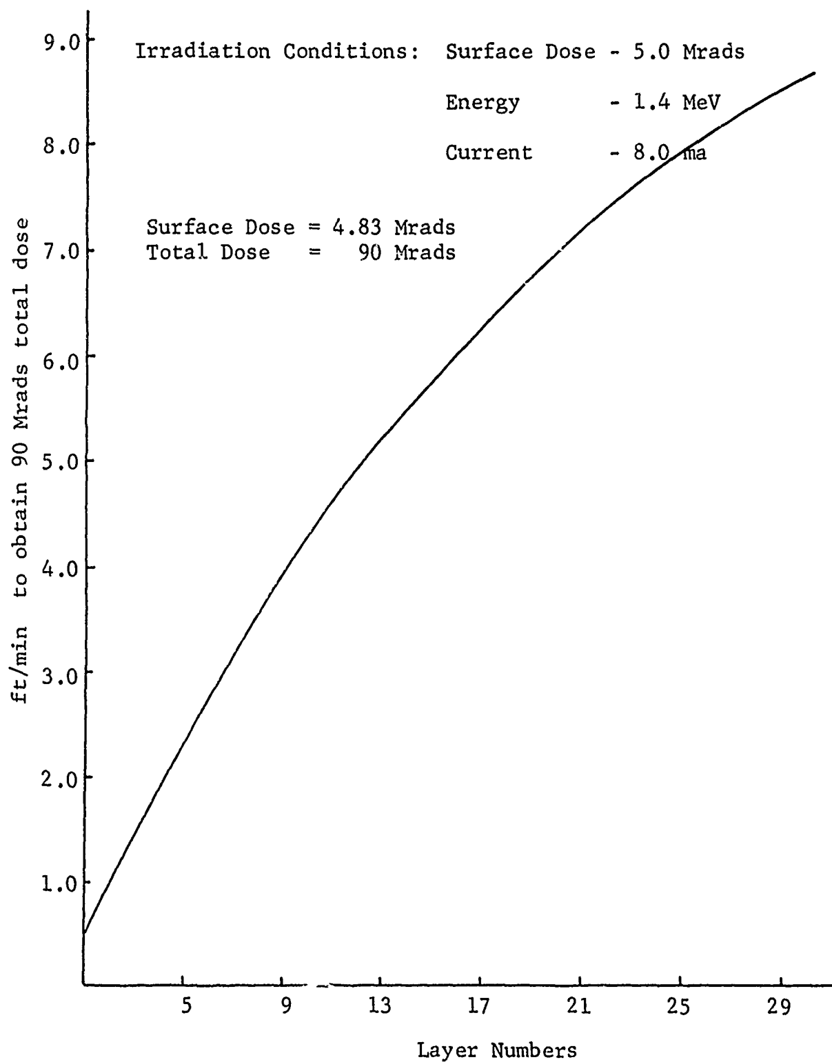
Figure 3-8 Film Velocity Needed For Travel Through a Given Number of Layers For 1 Mil Film With Layers Spaced 1 Inch Apart
