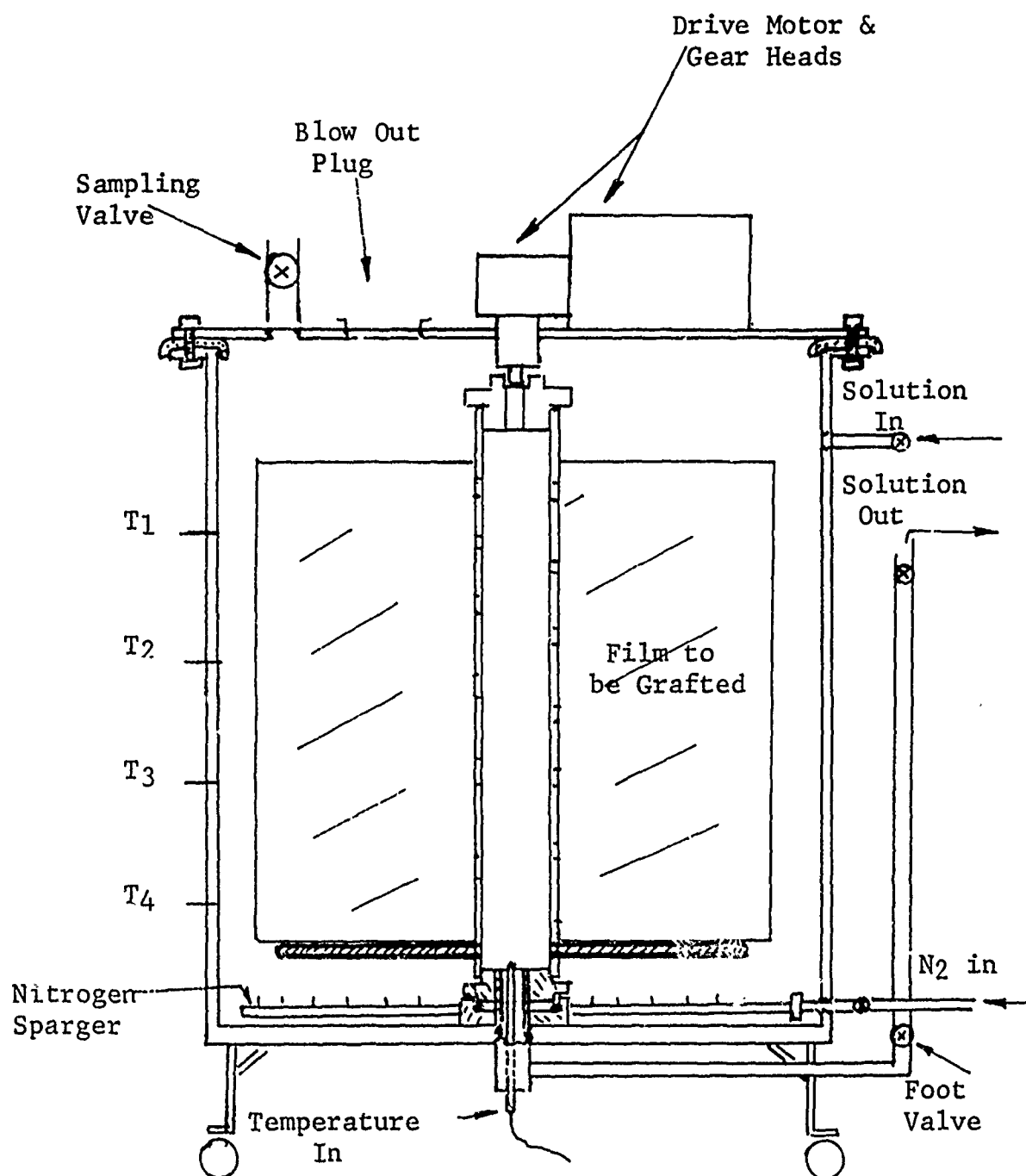
Figure 5-3. Schematic of Film Reactor
