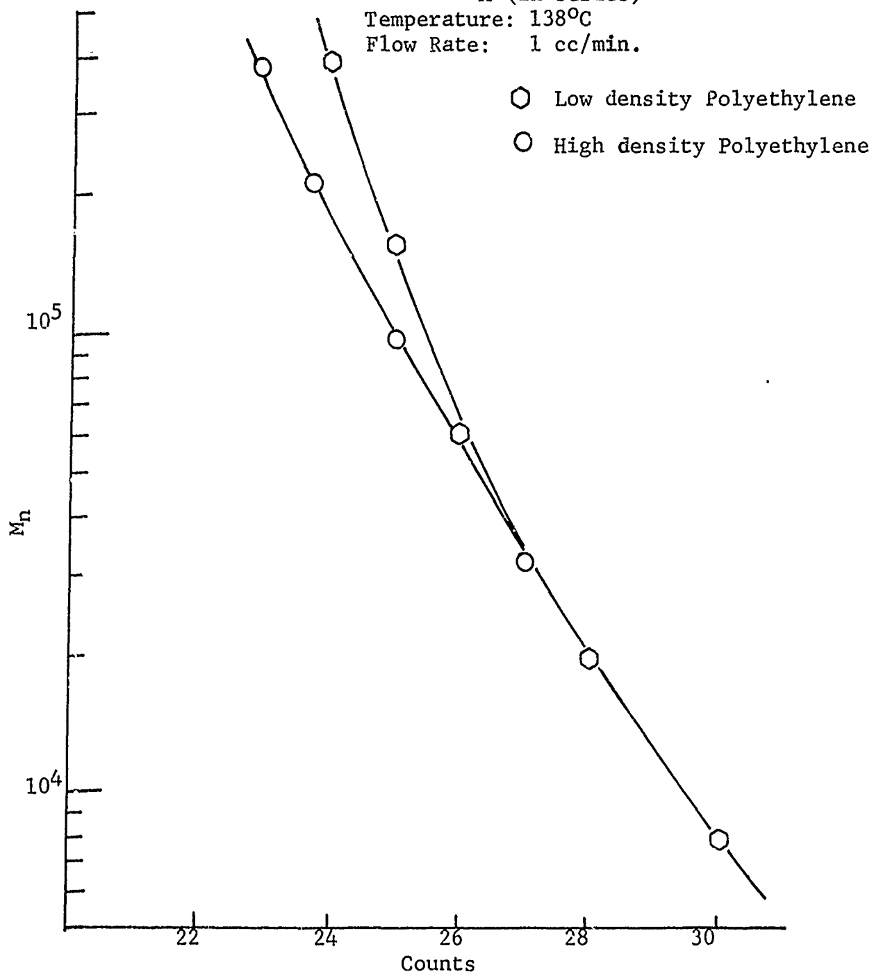
Figure 8-3. Standardization Curve for GPC.
