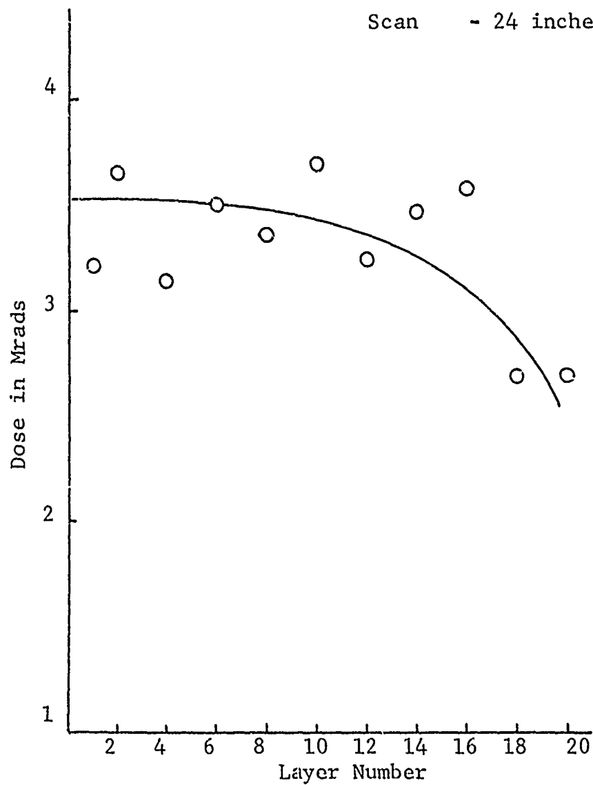
Figure 3-19 Dose-Layer Curve For 20 Layers of Three Mil Film
