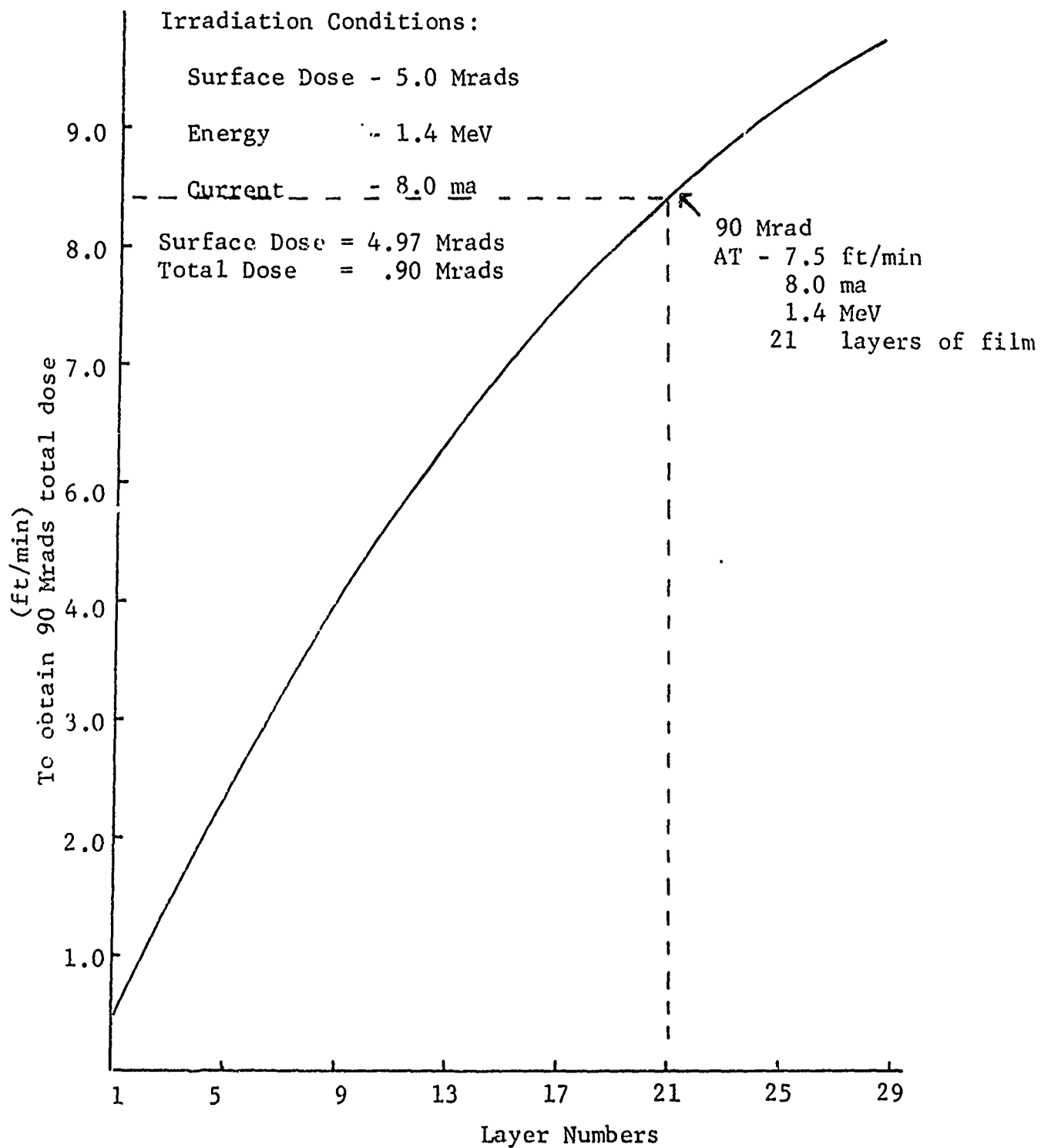
Figure 3-9 Film Velocity vs Number of Layers Required to Obtain 90 Mrads Total Dose For 2 Mil Film Spaced 1 Inch Apart
