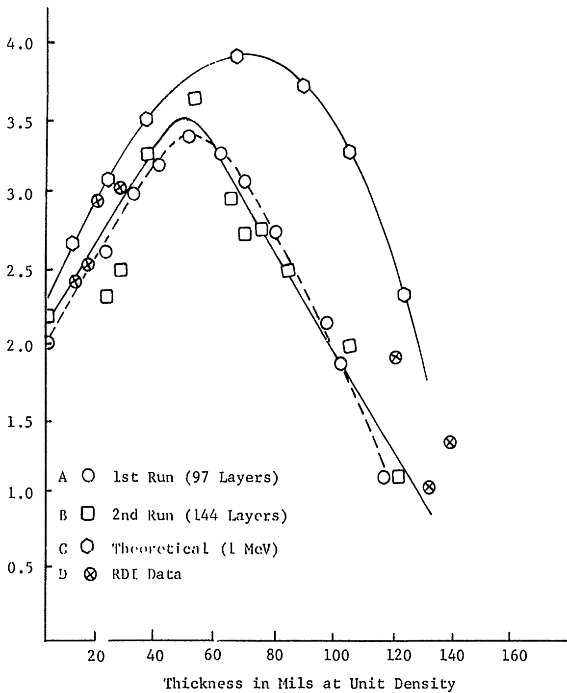
Figure 3-1 Theoretical and Actual Dose-Depth Curves
