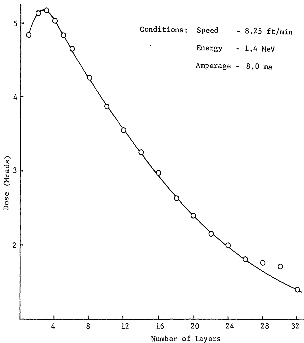
Figure 3-5 Dose Layer Curve for Arrangement of 1 Mil Film Spaced 1 Inch Apart Passing an Electron Beam
