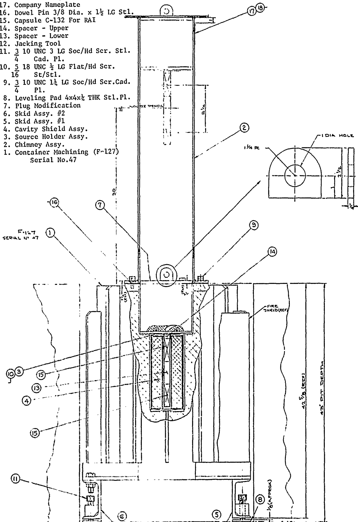
FIGURE 2-3 Cobalt 60 Source Cask and Guide Tube Assembly
