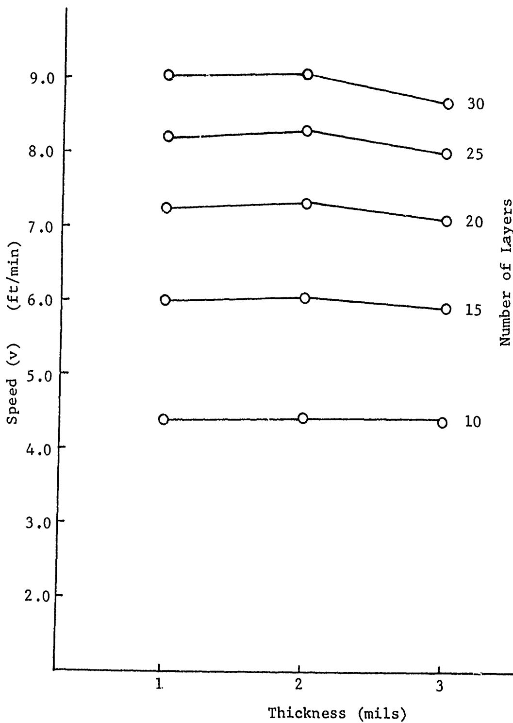
Figure 3-11 Speed vs Film Thickness With Number of Layers as a Parameter to Achieve 90 Mrads Total Dose
