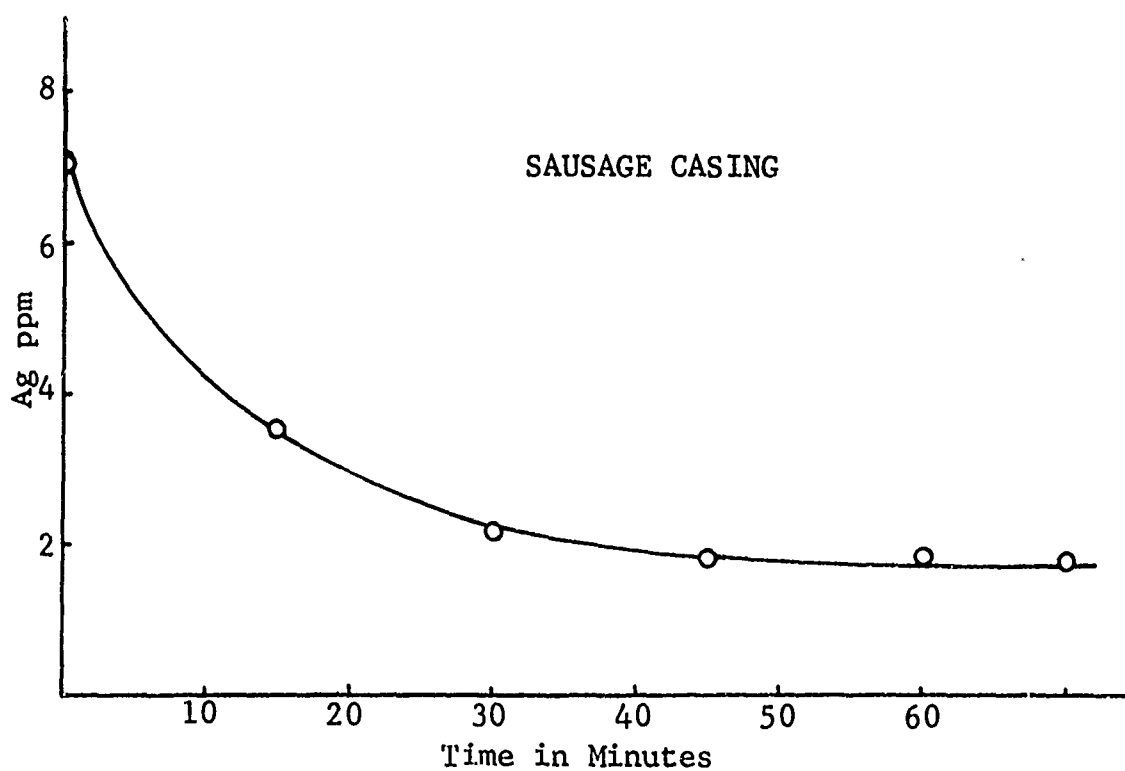
Figure 8-27. Silver Pick-up Through Membranes Silver Rich Side.
