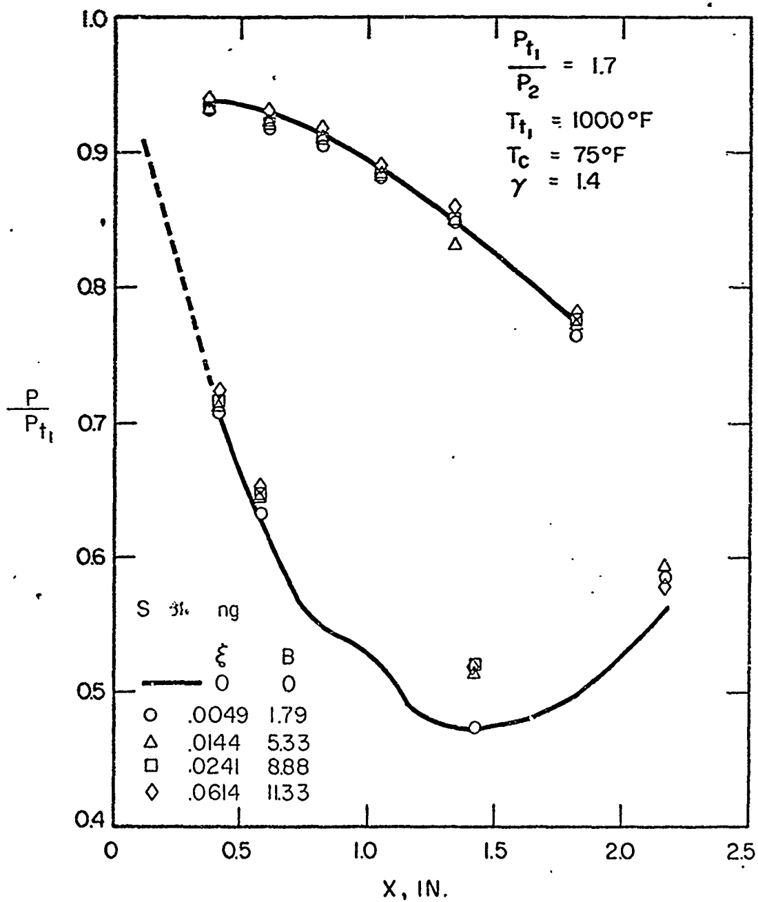
Fig. 28 - Static pressure profiles at P_{t1}/P_2 = 1.7 for S blowing on Model IV (30° chordwise blowing)
