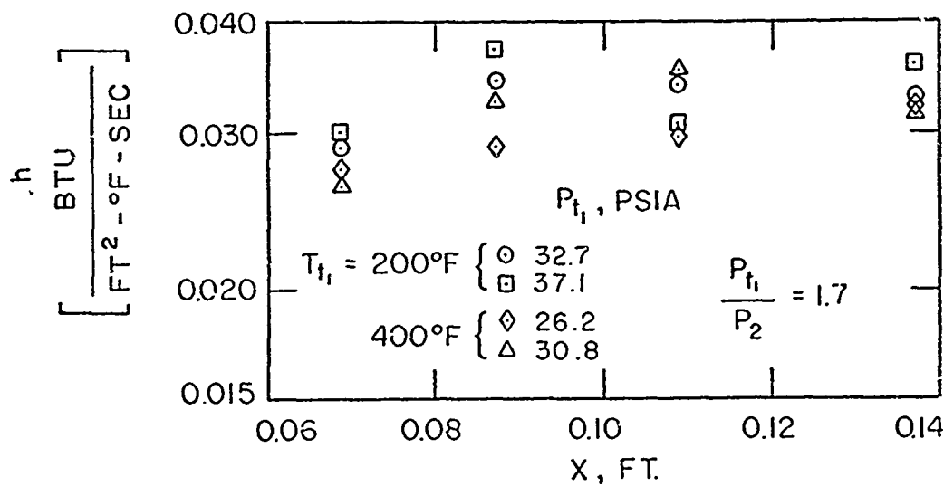
(b) P_{t_1}/P_2 = 1.7
