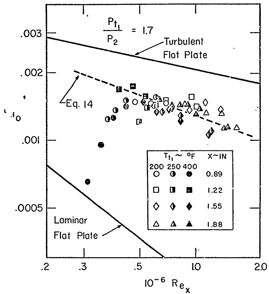
Fig. 39 - No-blowing Stanton number data for transonic suction surface
