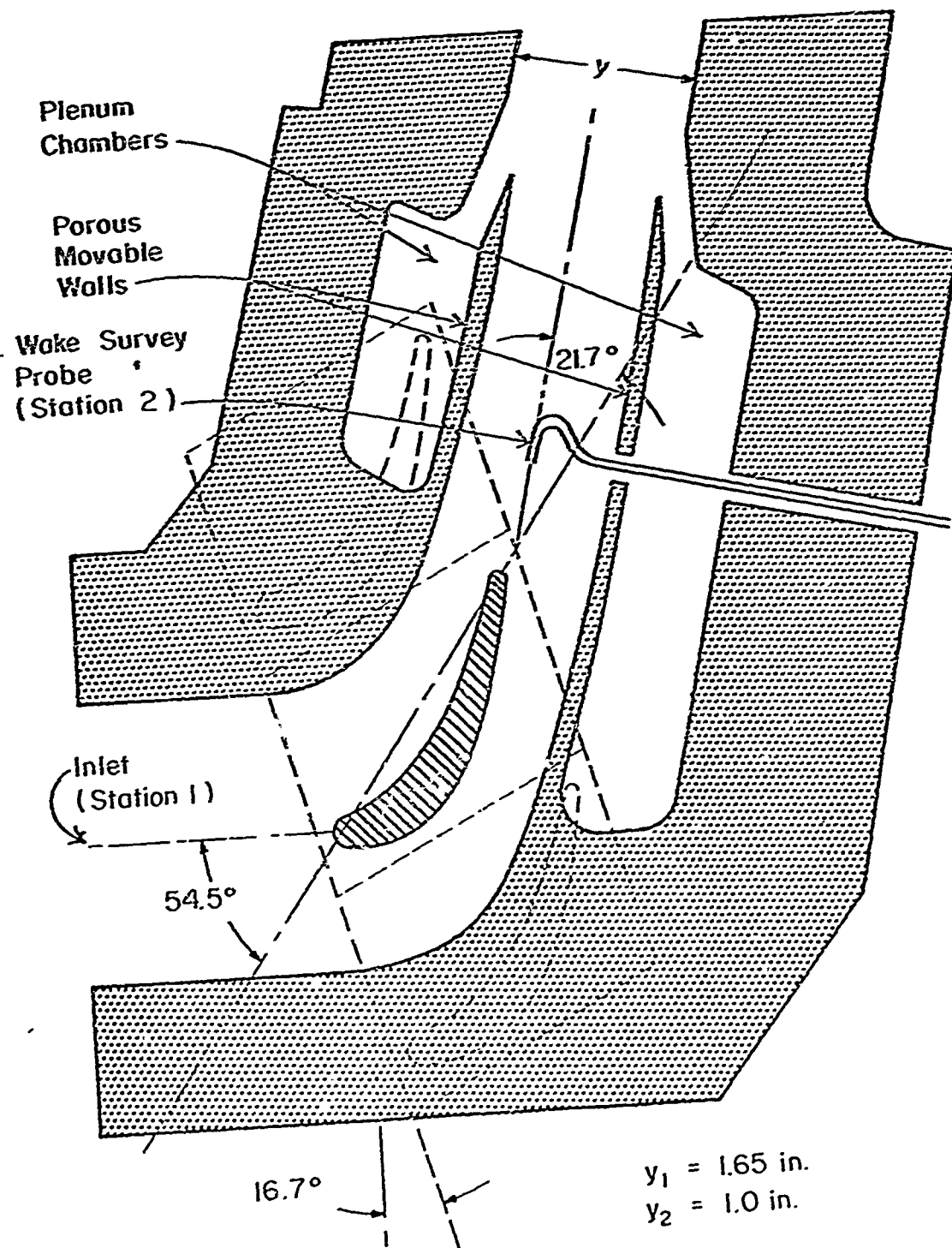
Fig. 2 - Profile of test cabin and related cascade
