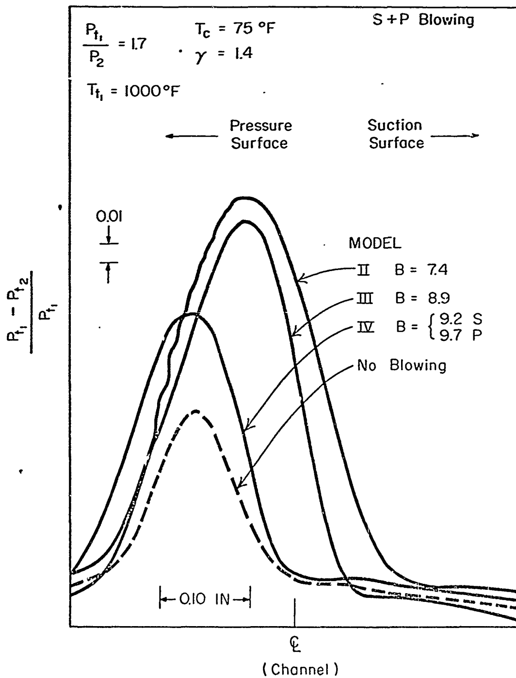
Fig. 31 - Typical wake total pressure surveys for massive blowing at P_{t1}/P_2 = 1.7
