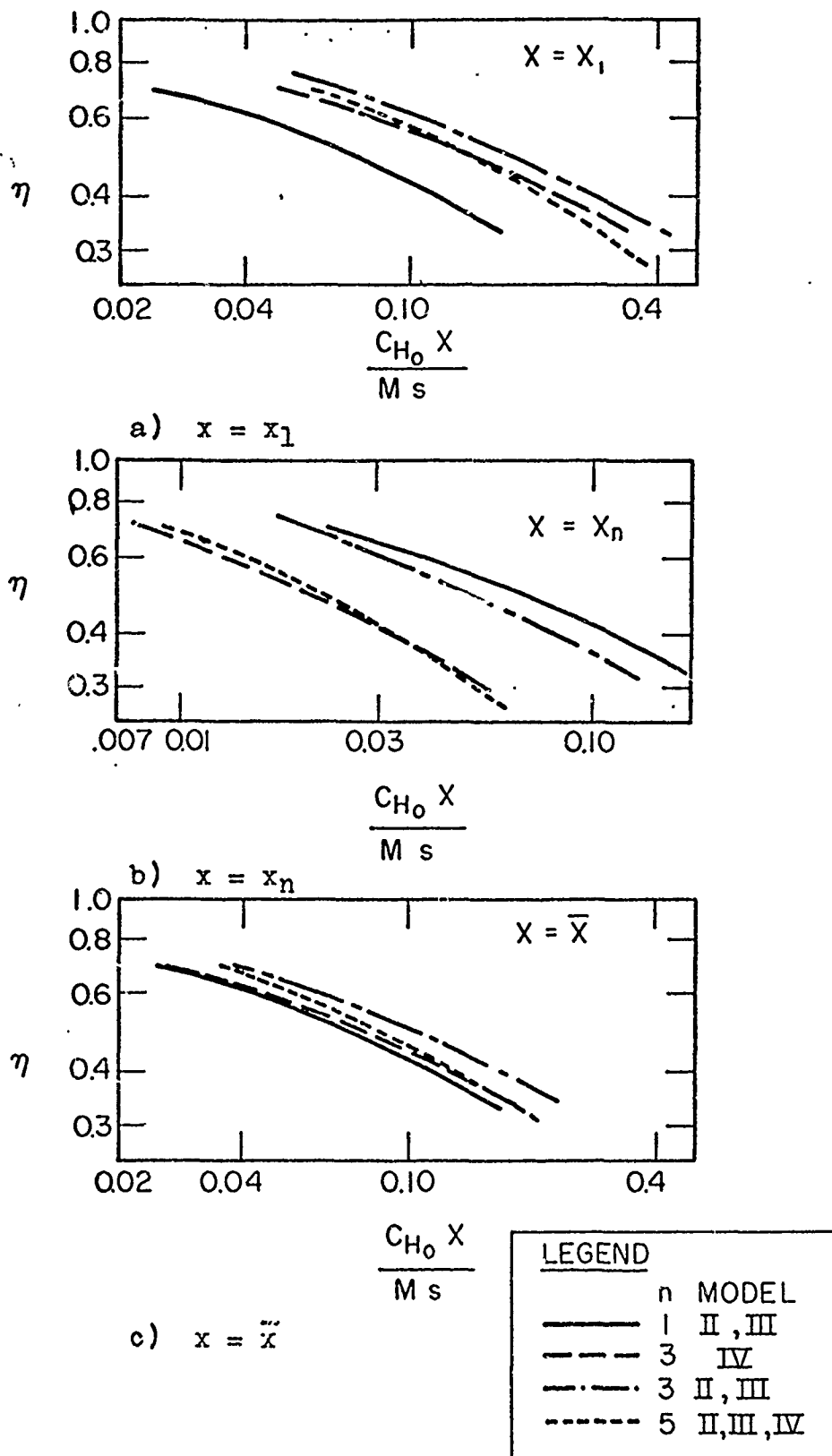
Fig. 52 - Present S + P suction surface data correlated by (a) x = x_1 , (b) x = x_n , (c) x = \bar{x}
