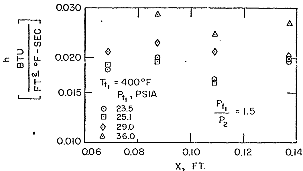
(a) P_{t_1}/P_2 = 1.5
