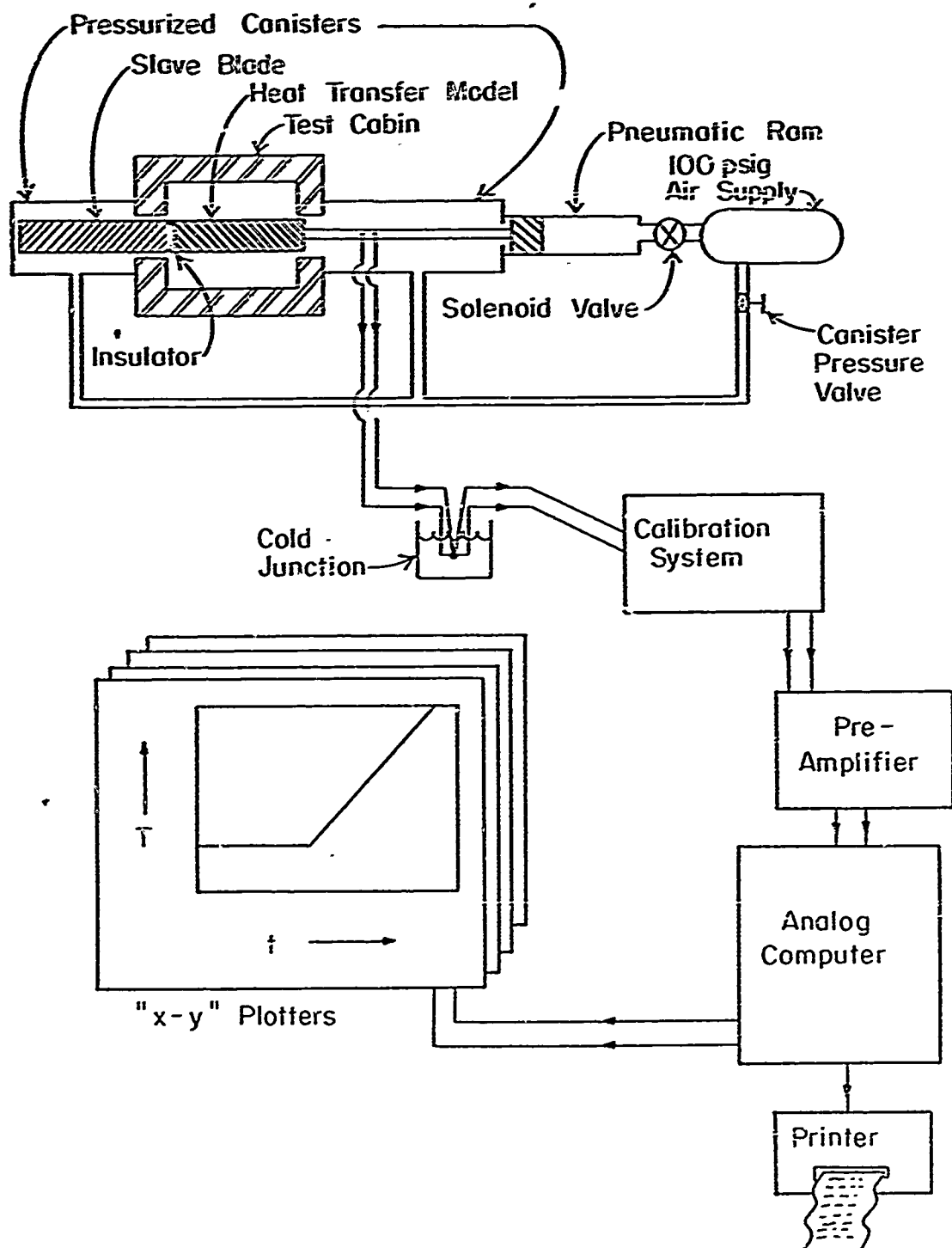
Fig. 14 - Schematic of heat transfer measurement system
