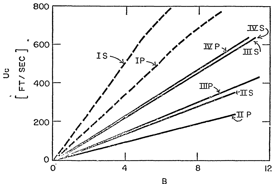
Fig. 17 - Nominal coolant velocities for film-cooling model surfaces
