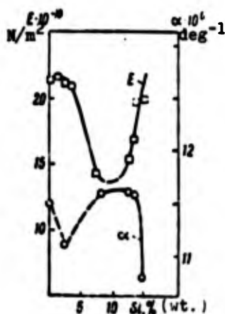
Fig. 2. Isotherms of modulus of normal elasticity E and the coefficient of thermal expansion \alpha of solid solutions at 20^\circ C .
