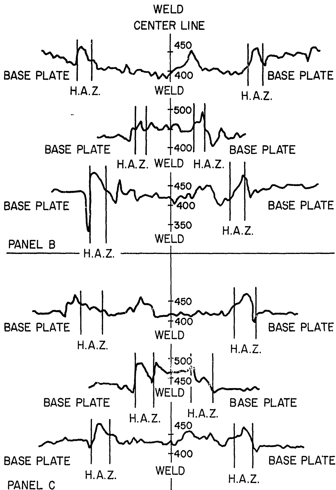
Fig. 5 -- Typical hardness (DPH) profiles
