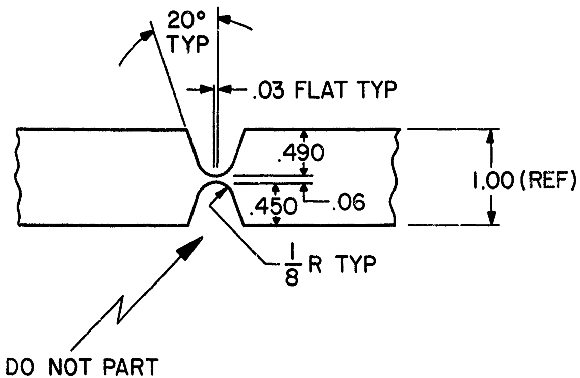
Fig. 1 - Weld preparation
