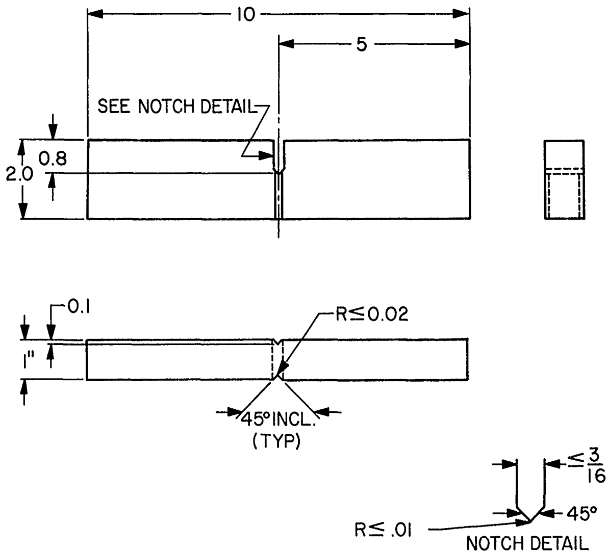
Fig. 7 - Notched-bend fracture specimen
