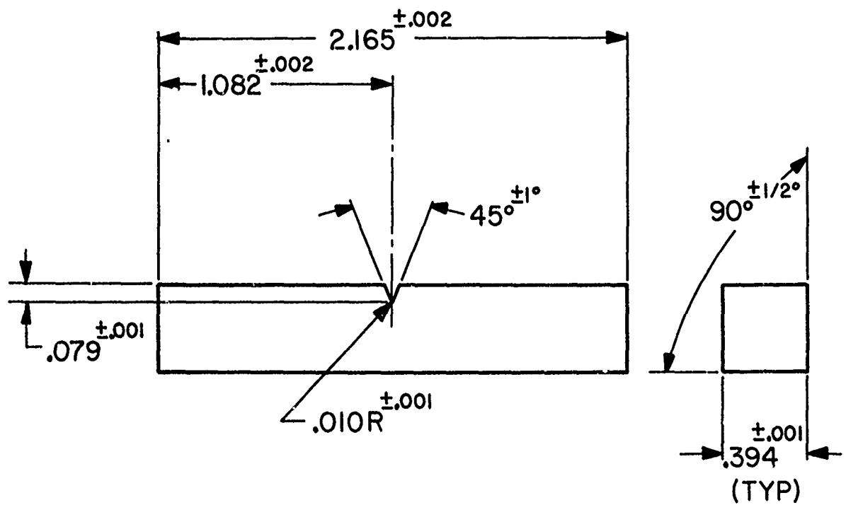
Fig. 3 Standard Charpy impact specimen
