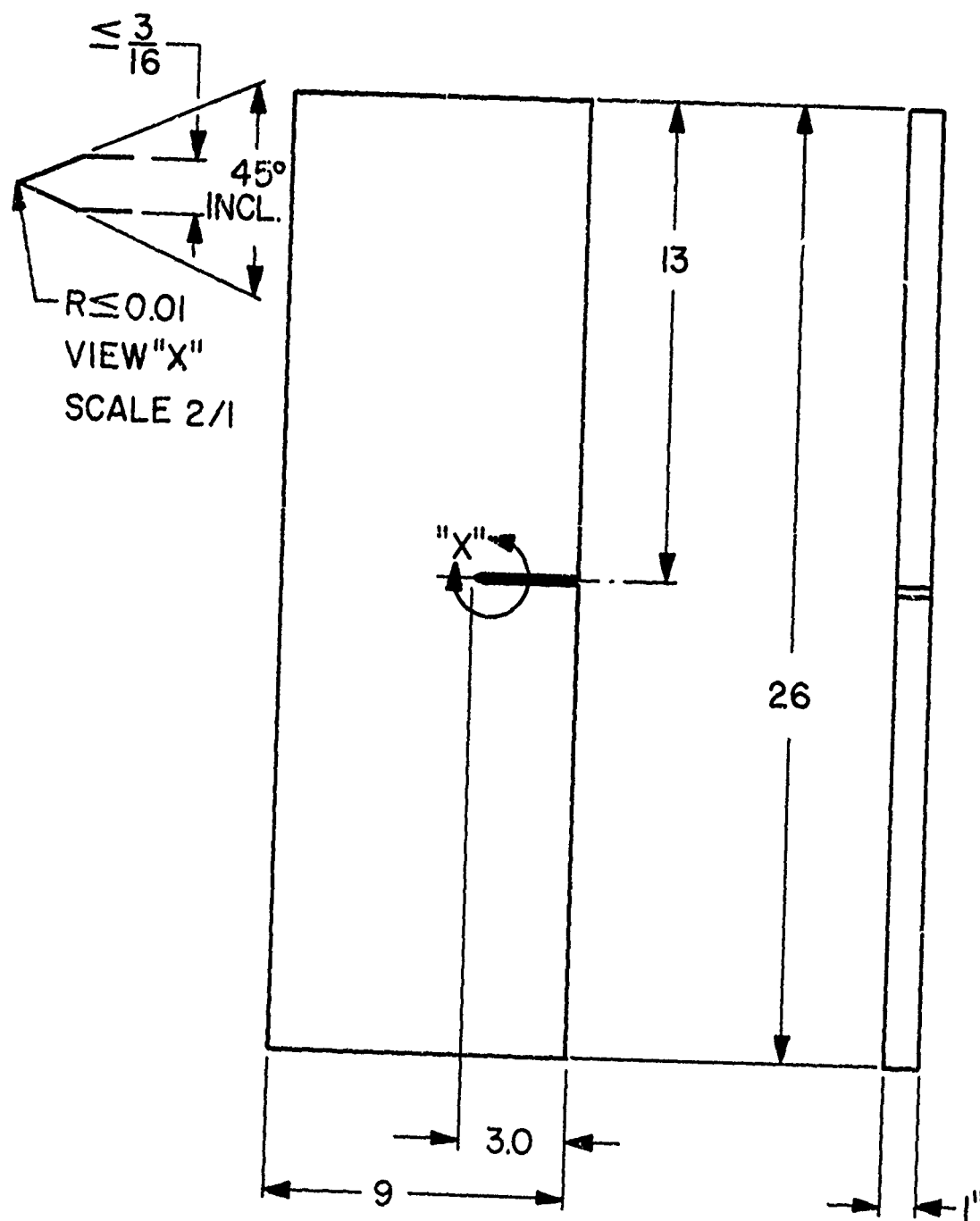
Fig. 6 - Large base-plate fracture specimen
