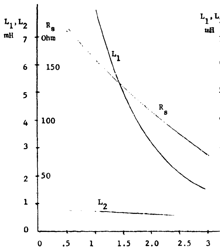
Fig14- Butterworth synthesis
