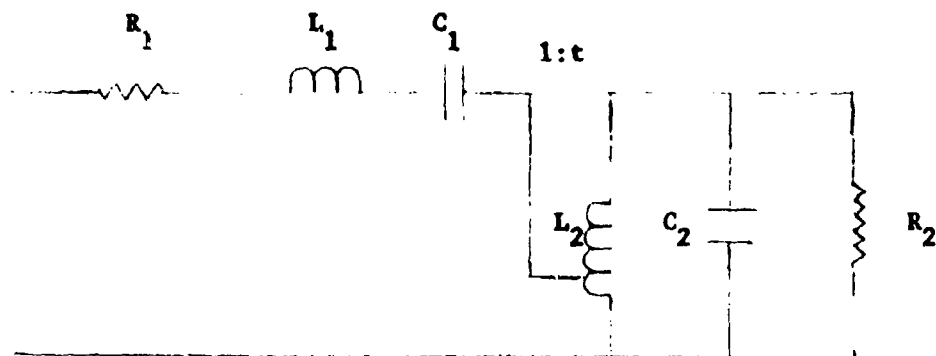
Fig. 19 - Band pass Bessel filter with ideal transformer
