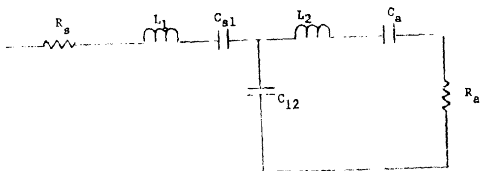
Fig 13 - Configuration of band-pass filter network
