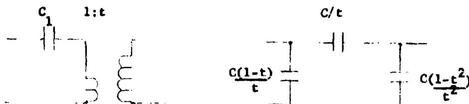
Fig.20- Example of Norton equivalent network transformation
