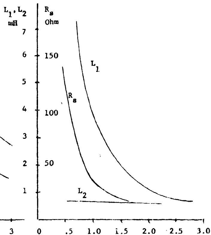
Fig15- Bessel synthesis
