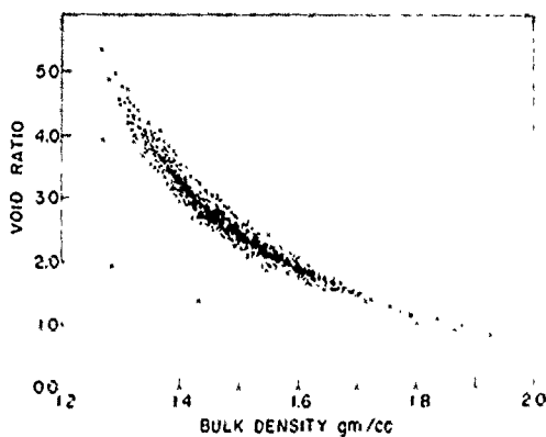
Fig. 10 - Bulk density vs void ratio for all data.
