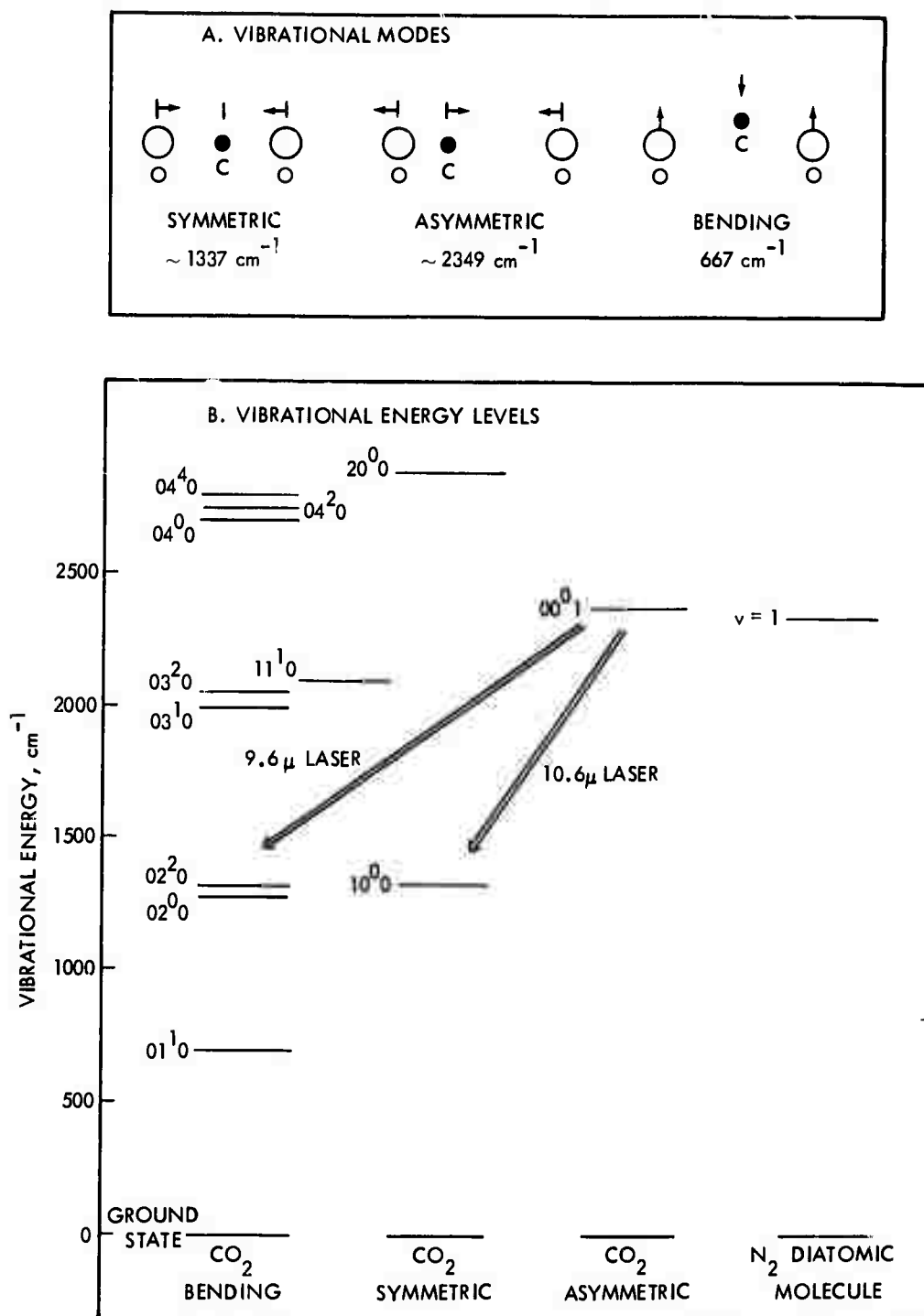
FIGURE 2. Vibrational Modes of \text{CO}_2 and \text{N}_2 Molecules Important in Gas Laser Operation. (Rotational states and many higher levels of excitation of the molecules are not shown.)
