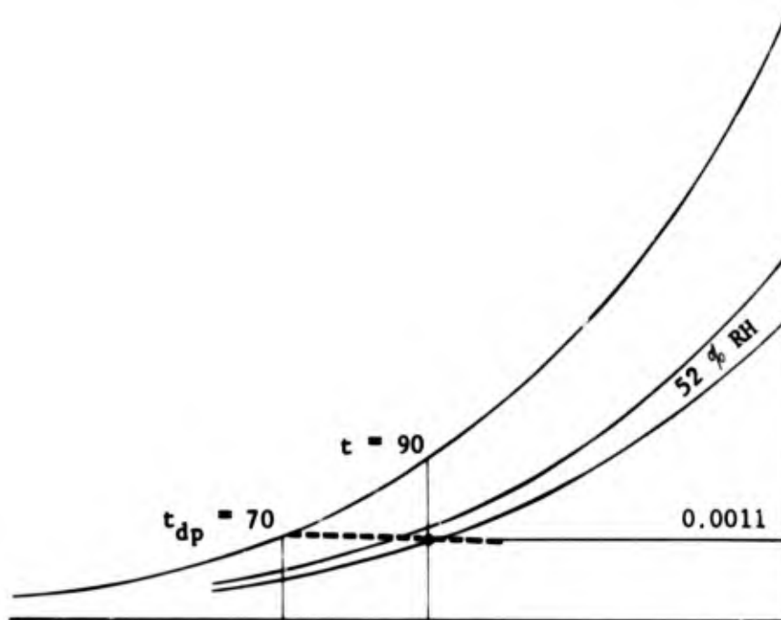
FIGURE 3. ILLUSTRATION OF A HUMIDITY PROBLEM
