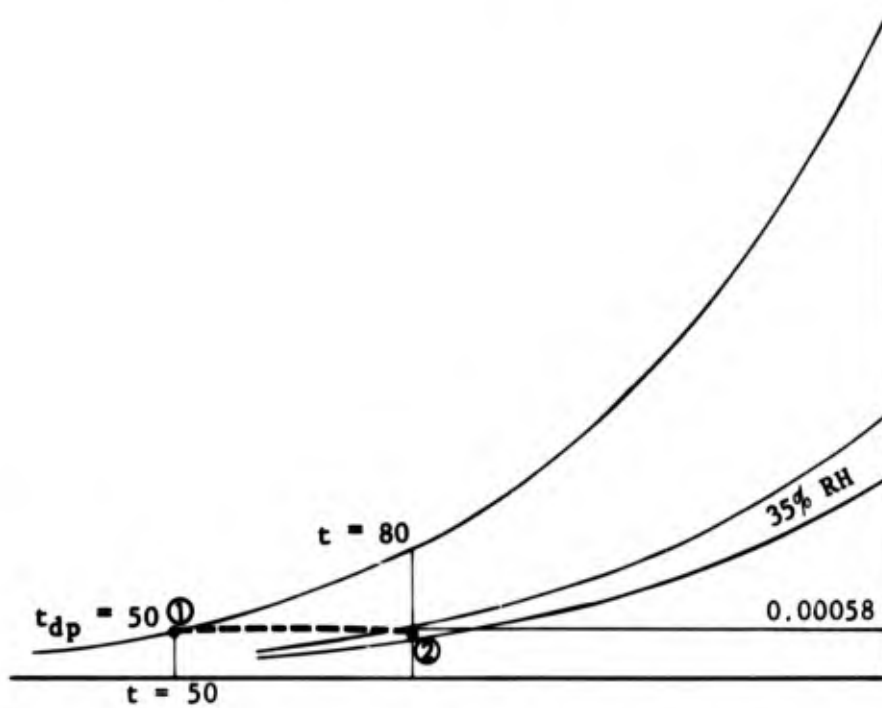
FIGURE 4. ILLUSTRATION OF A HEATING PROBLEM
