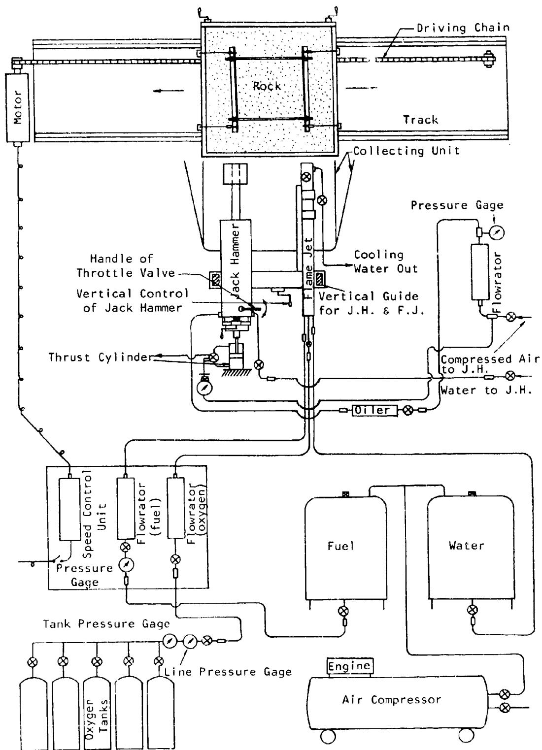
Fig. 50. Schematic of Experimental Apparatus for Thermo-mechanical Fragmentation
