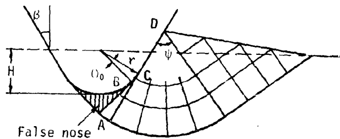
Fig. 31. Slip-line Fields for Indentors No. 3 and No. 4 for \phi = 0^\circ
