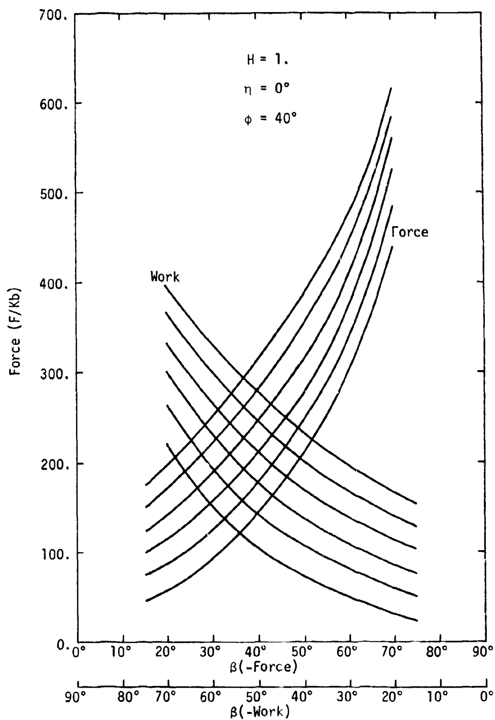
Fig. 42. Force-Angle Diagram for Indentors No. 1 and No. 2 for H = 1. , \eta = 0^\circ , and \phi = 40^\circ
