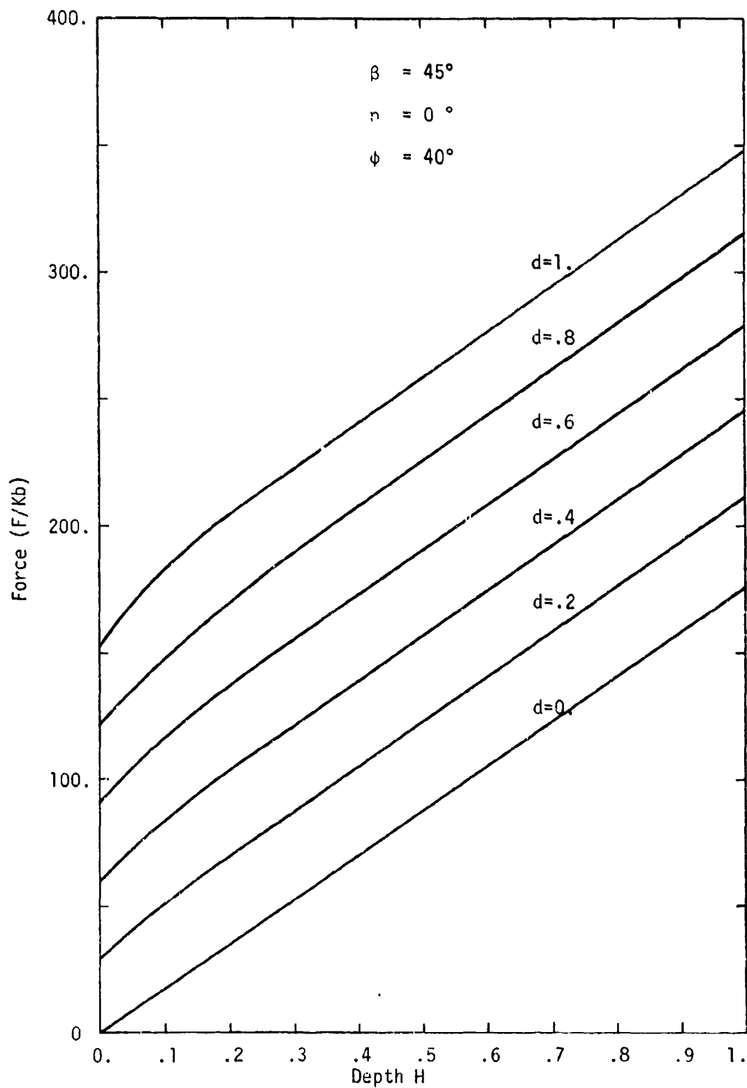
Fig. 40. Force-Depth Diagram for Indentors No. 1 and No. 2 for \phi = 40^\circ , n = 0^\circ and \beta = 45^\circ
