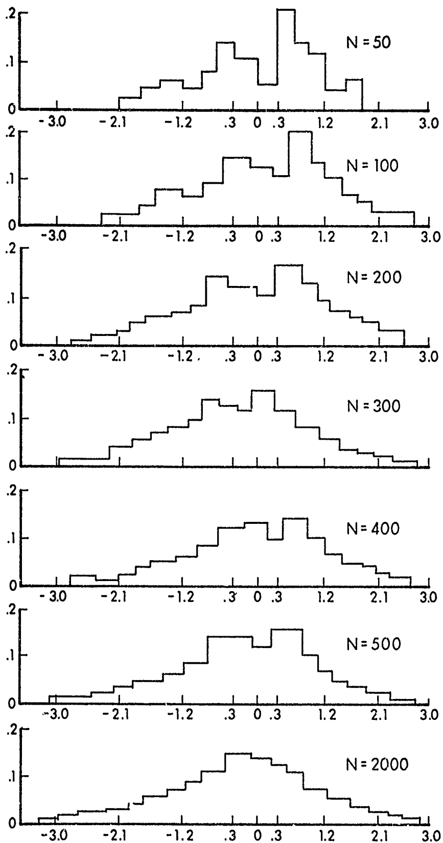
Figure 3.1 Frequency Histograms.
