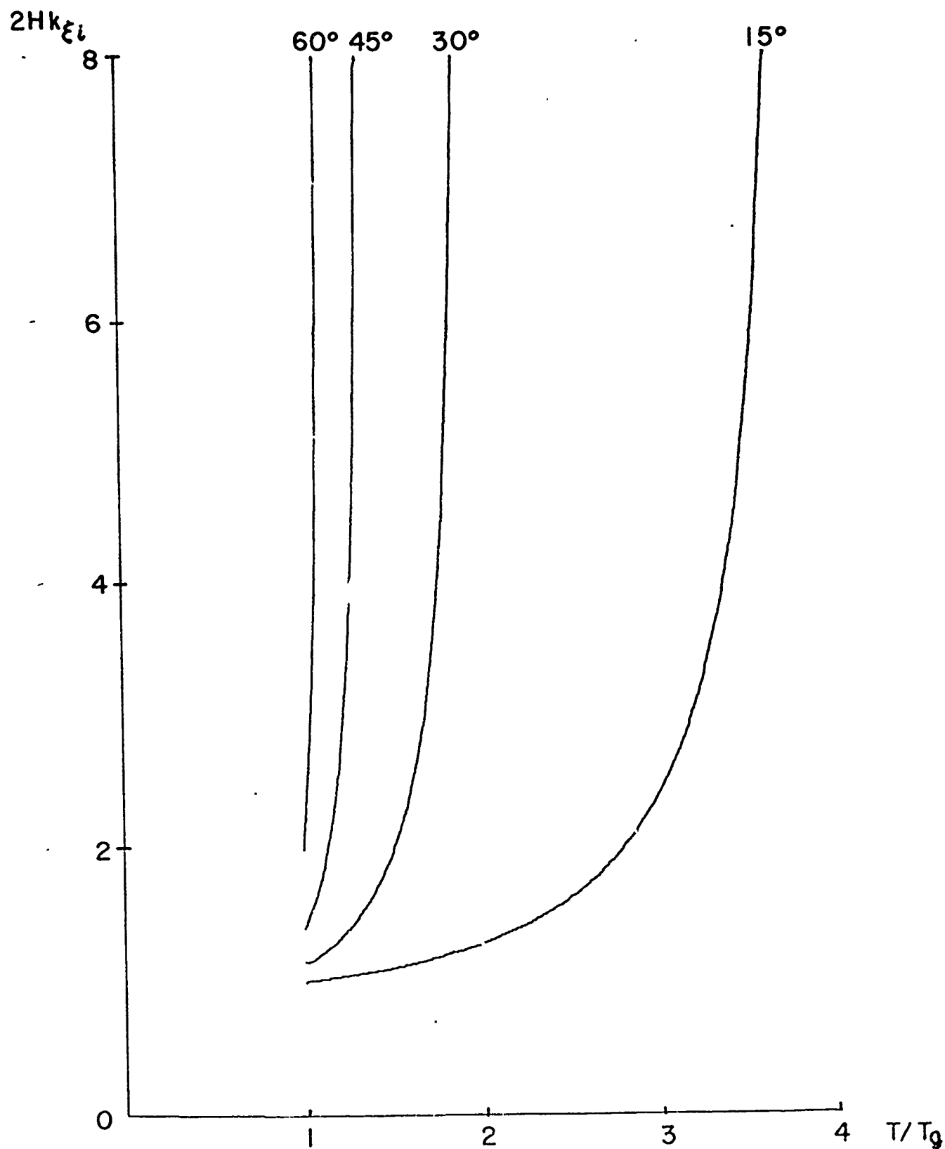
FIGURE 5 GRAPH OF k_{\xi i} / (1/2H) VS PERIOD T/T_0 WITH ANGLE \alpha AS PARAMETER
