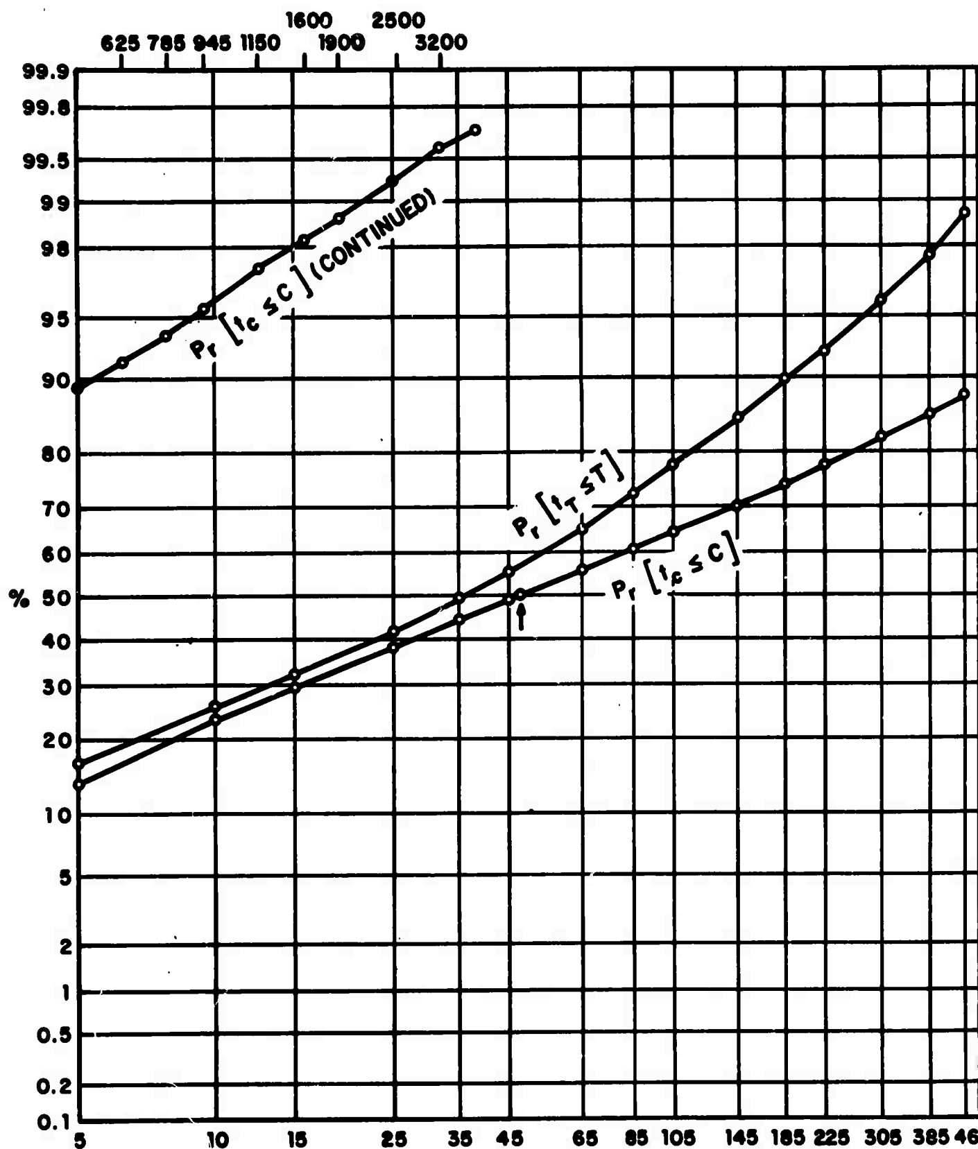
FIG. 8 CUMULATIVE P(T) and P(C)
