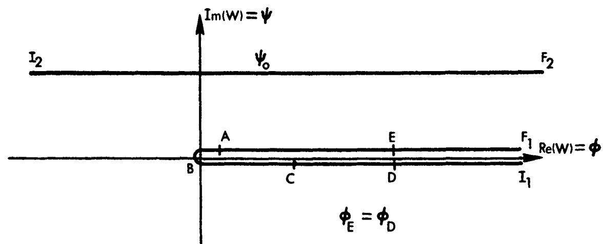
Figure 2. The Complex Potential Plane
