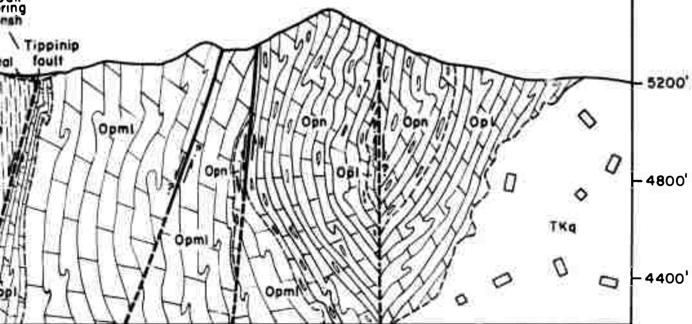
SECTION C-C'
