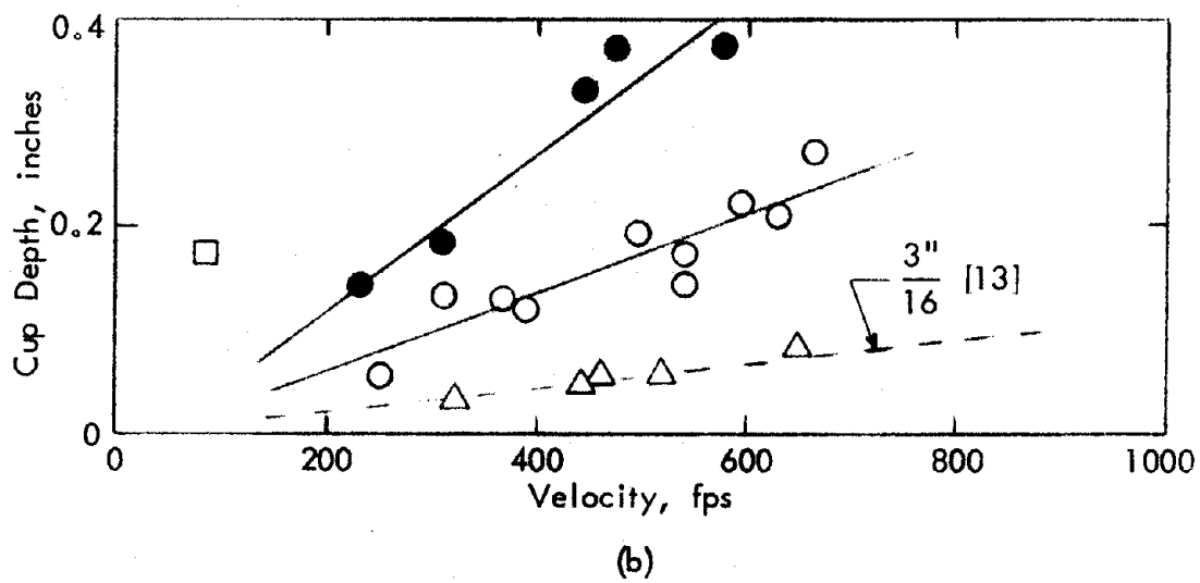
Fig. 11 - Penetration and Cup Depth for Berea Sandstone - Steel Spheres
