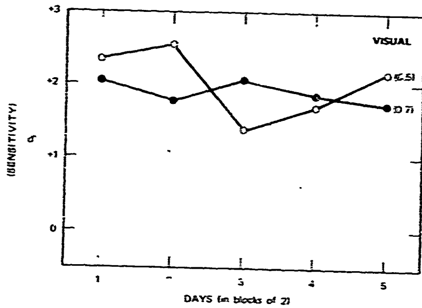
FIGURE 5 CHANGES IN d' OVER DAYS WITH A PRIORI PROBABILITIES AS A PARAMETER
