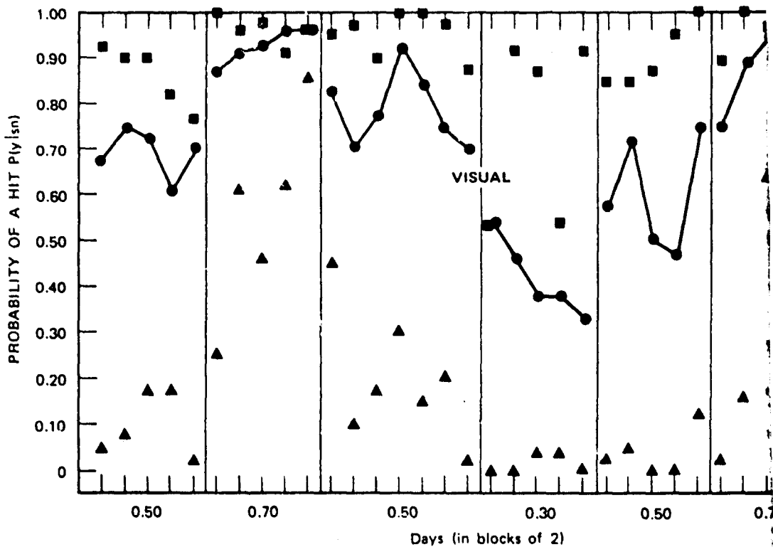
FIGURE 1 ACQUISITION OF CORRECT DETECTIONS OR HITS BY SEA LIONS AS A FUNCTION OF SIGNAL STRENGTH AND VARIATIONS IN THE A PRIORI PROBABILITY
