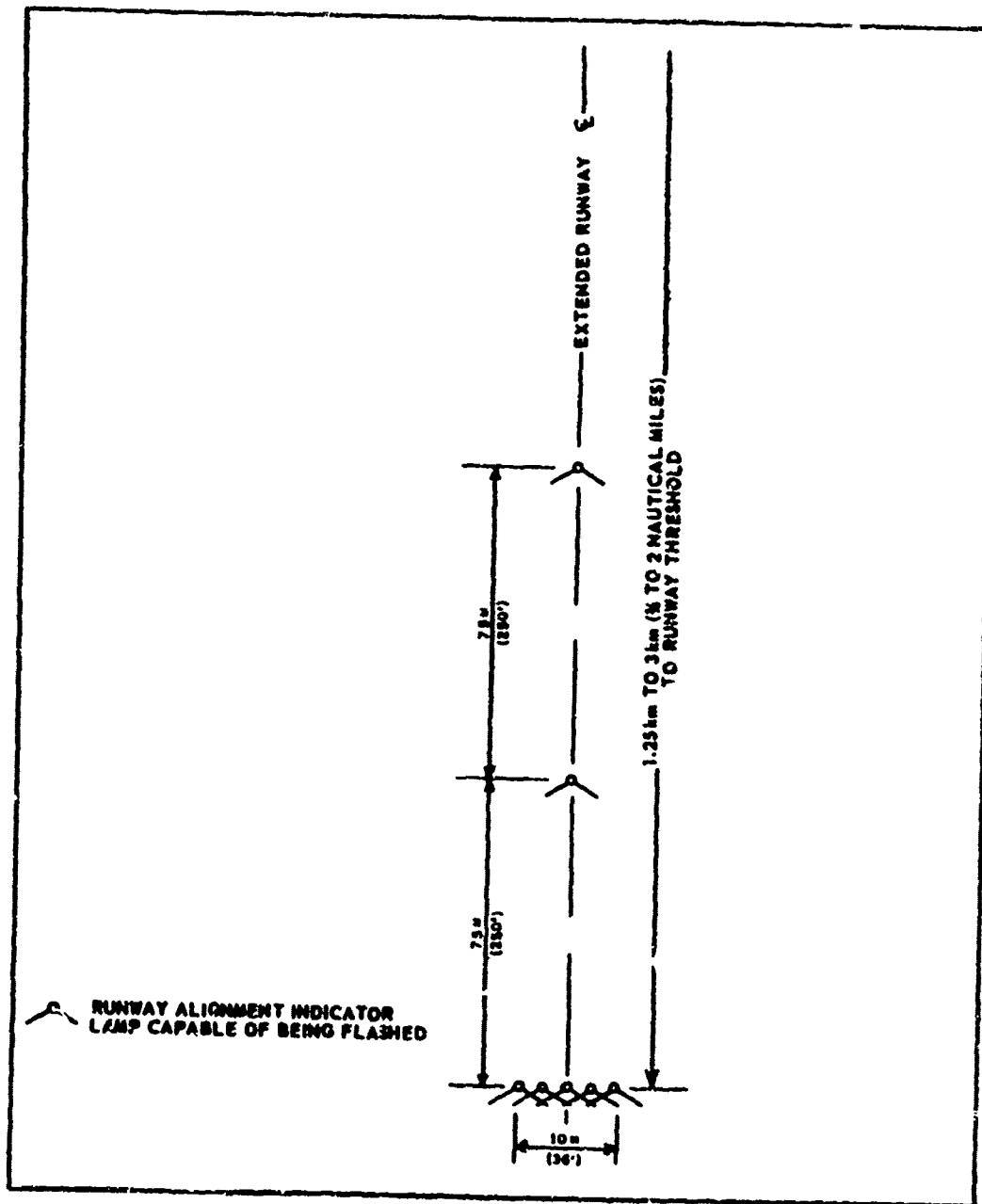
Fig. 2-3.- HIGH INTENSITY RUNWAY ALIGNMENT INDICATOR
