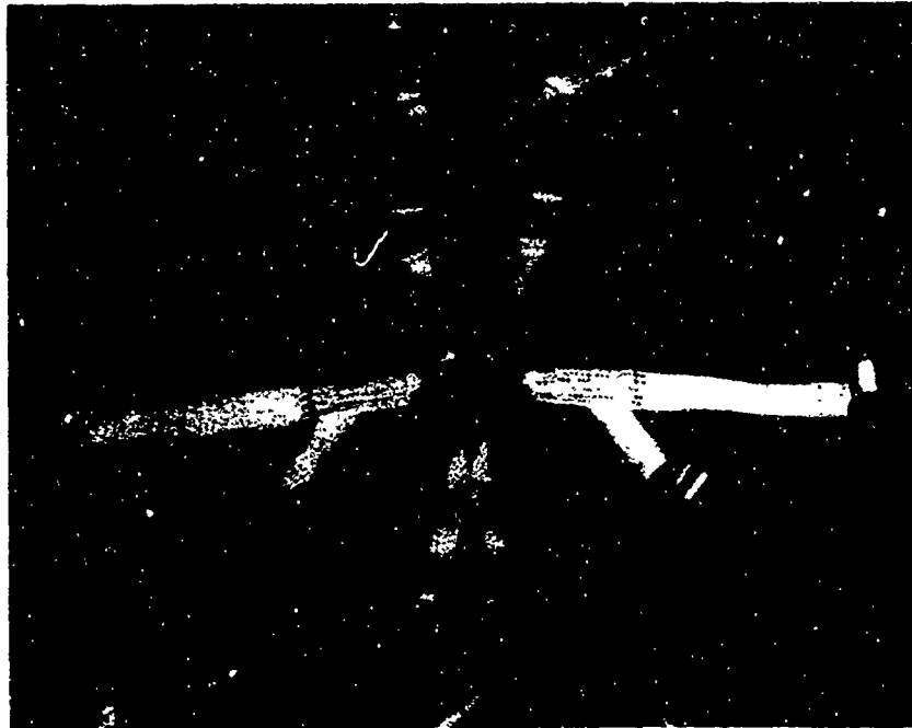
Figure 112. Posttest Frontal-End View of Restraint System.
