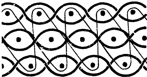
THREE-PLY PLAIN WITH 3/3 BINDERS
