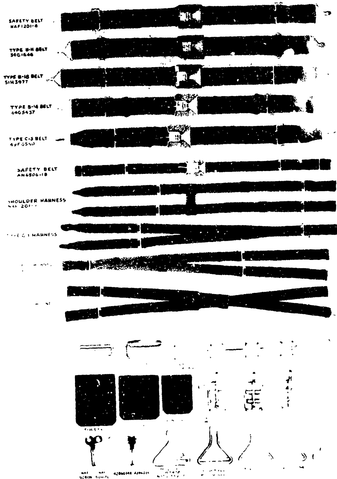
Figure 3. Existing Harnesses and Attachments.
