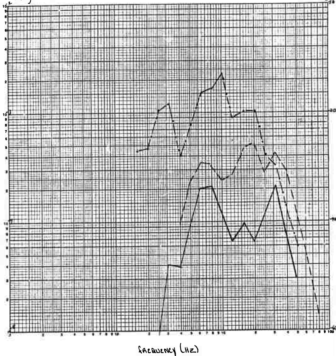
Figure 2-6. North Site, NTS, First P Motion
