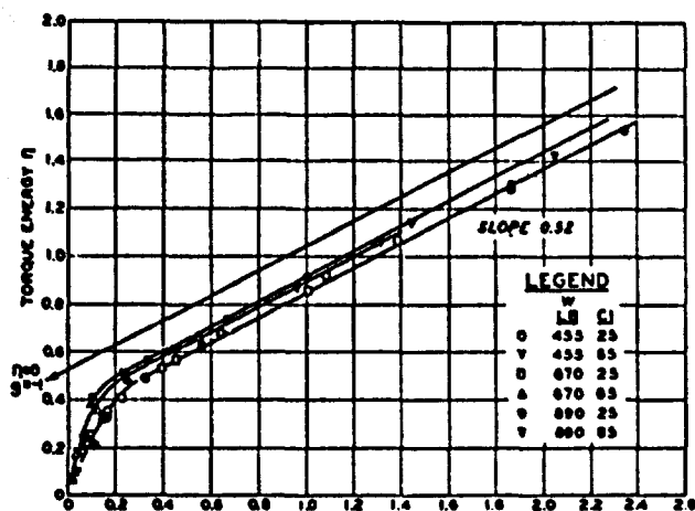
900-14, 2-PR TIRE 15% DEFLECTION
