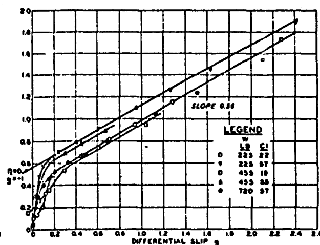
16-15-6R, 2-PR TERRA TIRE 25% DEFLECTION
