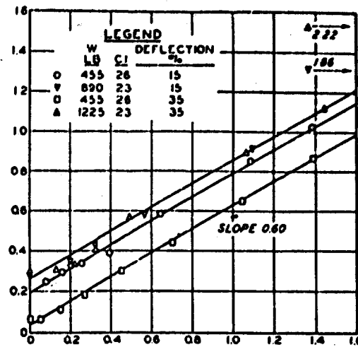
9.00-14, 2-PR TIRE CONE INDEX \approx 25
