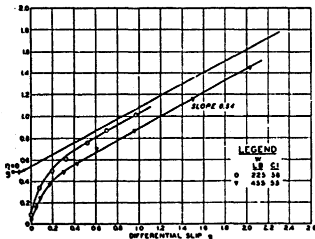
4.50-7, 2-PR TIRE 35% DEFLECTION
