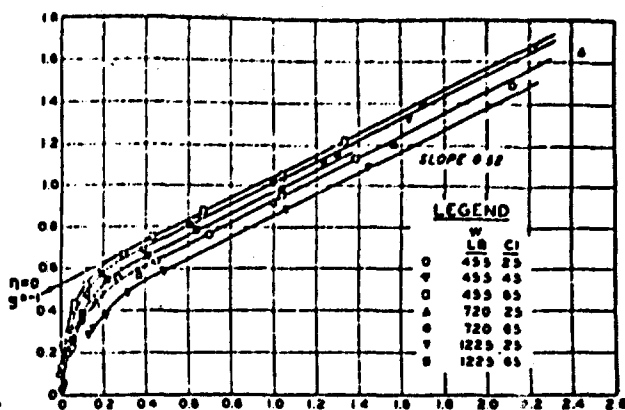
900-14, 2-PR TIRE 35% DEFLECTION
